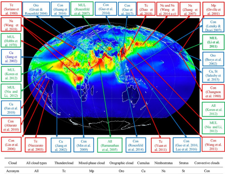
FIG. 14.4 A survey of observation-based studies of the effects of changes in aerosol on precipitation around the world sorted by location and cloud/precipitation regimes (Tc, Con, Mp, Oro, Cu, Ns, St, Con; acronyms defined in the plot). Colored text denotes enhanced (red), suppressed (blue) and dual effects (green) on precipitation by increases in aerosol.
