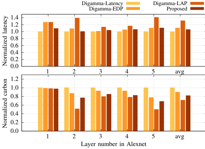
Fig. 4: Comparative analysis of normalized latency and embodied carbon for DNN accelerators designed for Alexnet using different optimization methods.
