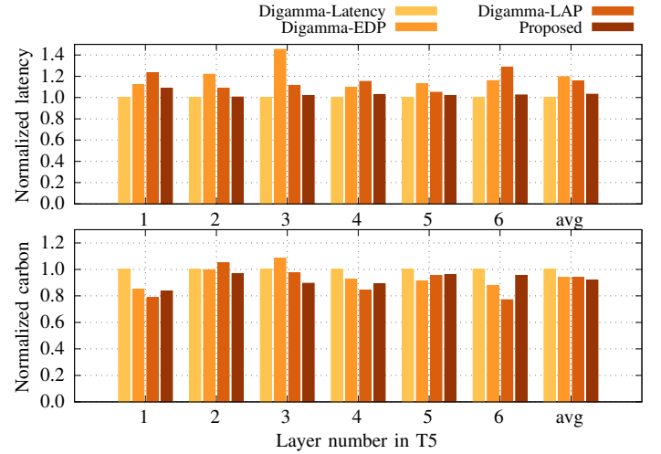
Fig. 7: Comparative analysis of normalized latency and embodied carbon for DNN accelerators designed for T5 using different optimization methods.
