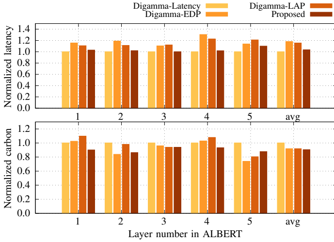
Fig. 5: Comparative analysis of normalized latency and embodied carbon for DNN accelerators designed for ALBERT using different optimization methods.
