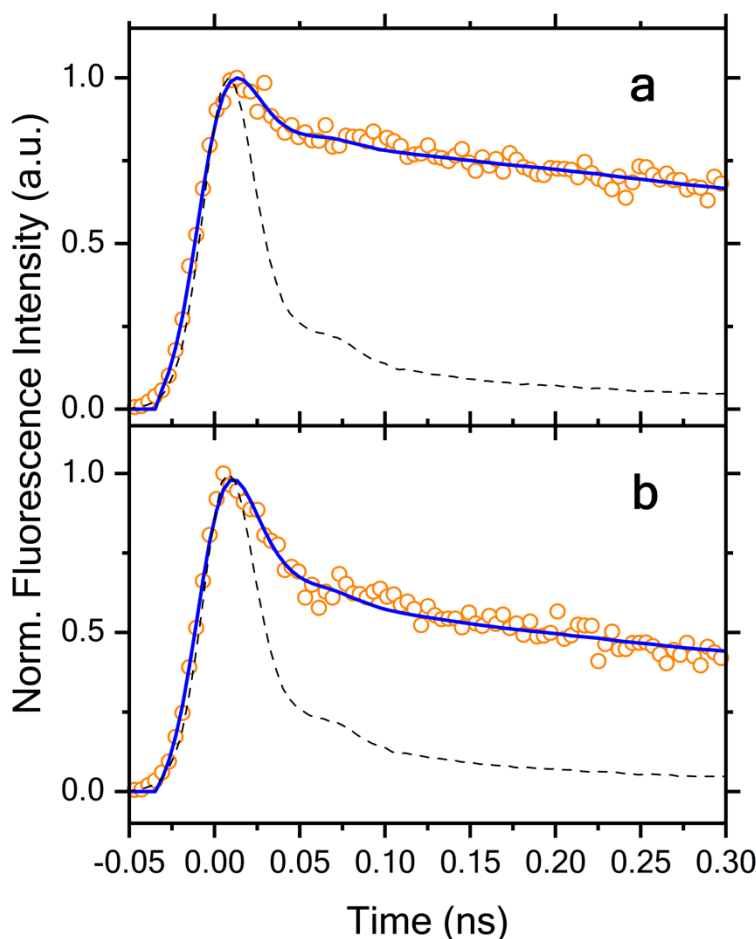
Figure 11. Early time portions of the time-resolved fluorescence decays acquired at 480 (a) and 540 nm (b), their corresponding deconvolution fits (solid lines) and the IRF (dash lines). The peak intensities of all these data are scaled to 1.0 for ease of comparison.
