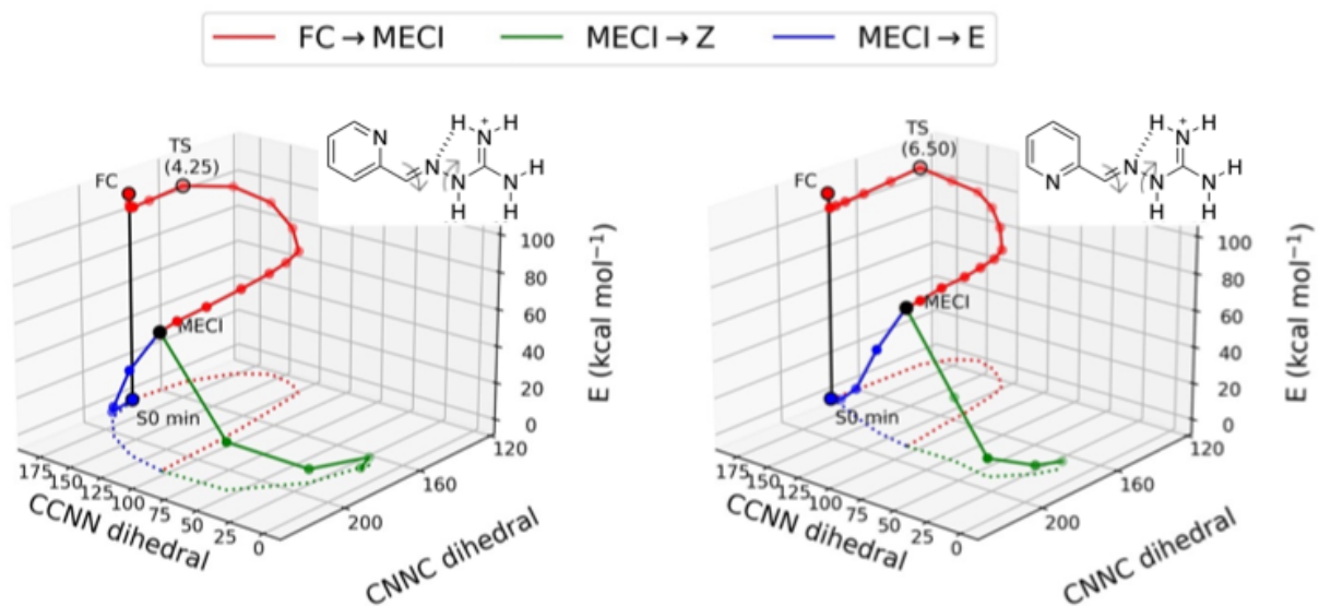
Figure 13. The reaction paths of the E_1 (left) and E_2 (right) conformers of 2PyMIG-HBr are shown starting from the Franck-Condon geometry. The reaction proceeds downward in energy to the S_1 minimum, then over a transition state and diverges to the possible photoproducts at the MECI. Dotted lines show the projection of the reaction to path onto the CCNN and CNNC dihedrals. Dihedral angles are identified in the insets. Transition state nodes are labeled as TS with the barrier from the S_1 minimum reported in kcal mol -1 .
