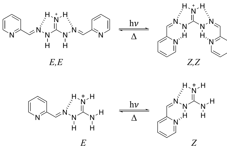
Figure 1. Structural changes of the 2PyDIG (top) and 2PyMIG (bottom) cations upon irradiation with UV light. Hydrogen bonds are noted as dashed lines.
