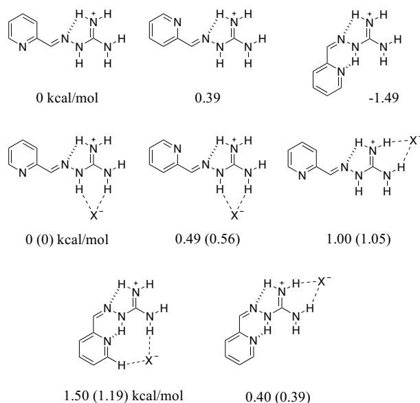
Figure 7. Relative free energies of the local minima of 2PyMIGH + and 2PyMIG-HCl(Br) at the DLPNO-CCSD(T)/aug-cc-pVTZ//M06-2X/def2TZVPP level, with solvent corrections included using the SMD solvation model for DMSO. Intramolecular hydrogen bonding and anion binding are noted as short and long dashed lines, respectively.
