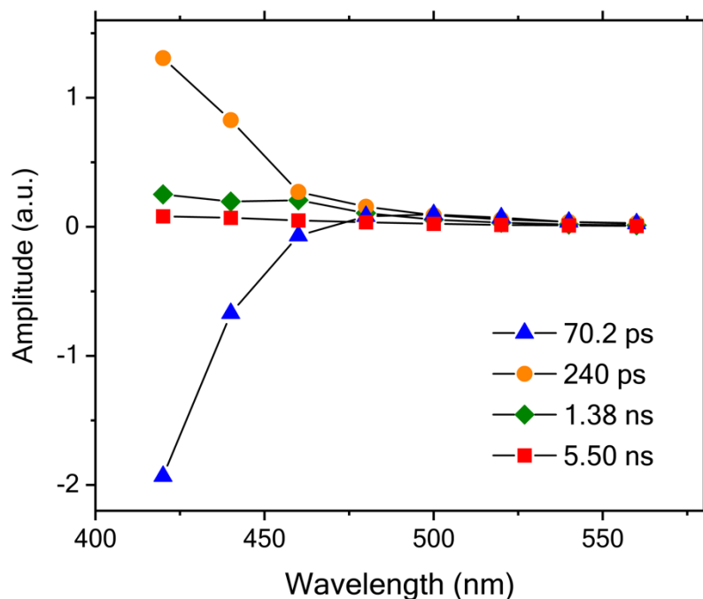
Figure 10. Decay associated spectra obtained for the time-resolved fluorescence kinetics measured at different emission wavelengths upon an excitation using laser pulses centered at 356 nm. The solid lines are guides to the eye.
