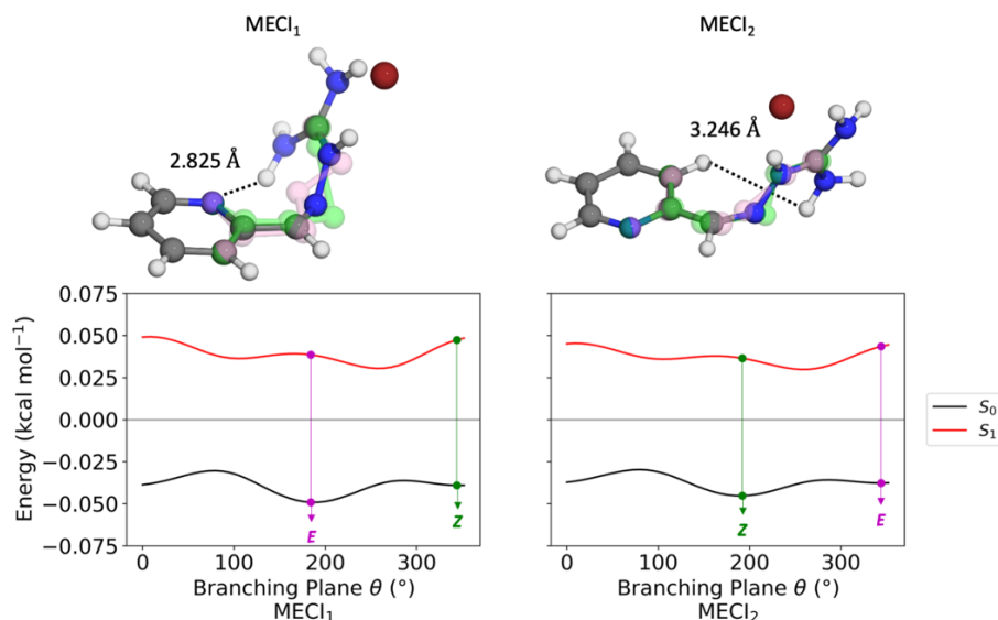
Figure 14. Geometries for MECI 1 and MECI 2 (top) are depicted along with the geometries corresponding to S_0 minima along the branching plane (step size = 0.4 a.u.) visualized in transparent pink (to E ) and transparent green (to Z ). The angle ( \theta ) between the derivative coupling
