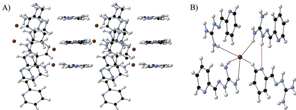
Figure 4. The crystal structure of 2PyMIG·HBr highlighting (A) the \pi -stacking motif of 2PyMIG cations and (B) the hydrogen bonding to the bromide anion (black dashed lines) and intermolecular hydrogen bonding between 2PyMIG cations (red dashed lines). Blue spheres are nitrogen atoms, black spheres are carbon atoms, and white spheres are hydrogen atoms.
