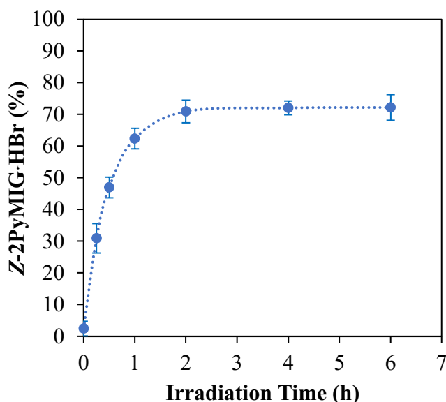
Figure 5. Conversion of 10.04 mM 2PyMIG-HBr from the open E form to the closed Z photoisomer over the course of 6 h under UV irradiation in DMSO- d 6 . Dotted lines are for visual aid.
