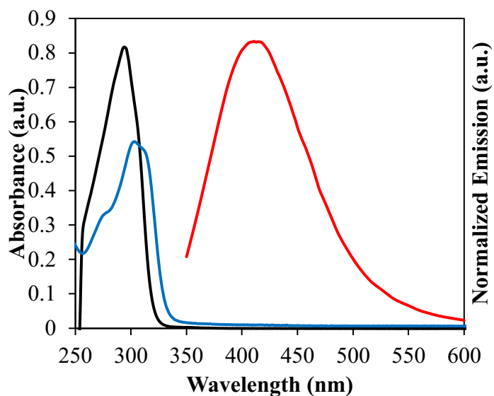
Figure 8. UV-Visible absorbance spectra of E -2PyMIG·HBr (black), Z -2PyMIG·HBr (blue), and the emission of E -2PyMIG·HBr at ( \lambda_{\text{ex}} = 315 nm, red).
