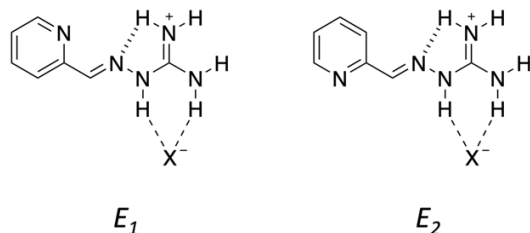
Figure 2. Starting E -conformers for the MECI searches are shown.
