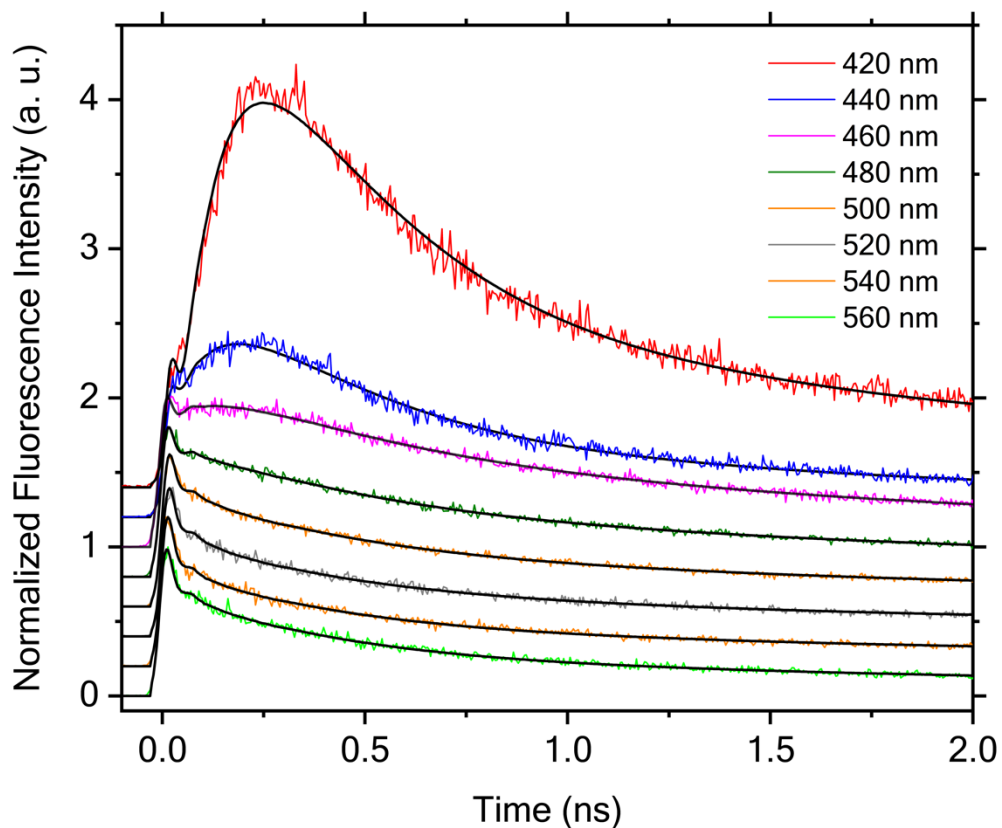
Figure 9. Time-resolved fluorescence kinetics measured at different emission wavelengths upon excitation with laser pulses centered at 356 nm. The peak intensities are scaled to 1.0 for all data except those measured at 420 and 440 nm, where the scaling was made for the initial shoulder
