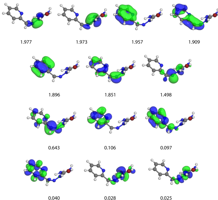
Figure 3. State-averaged natural orbitals (isovalue 0.05 a.u.) and occupations at MECI 1 calculated at the SA2-CAS(14,13)SCF/6-31G* level of theory.
