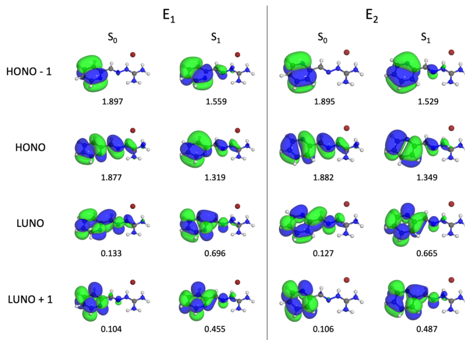
Figure 12. Frontier natural orbitals (isosurface 0.02 a.u.) of the E_1 (left) and E_2 (right) isomers and their occupations calculated from SA-CASSCF(14,13)/6-31G* are shown for the S_0 and S_1 surfaces.
