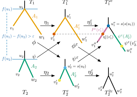
Fig. 7 An illustration for the proof of Proposition 1.
