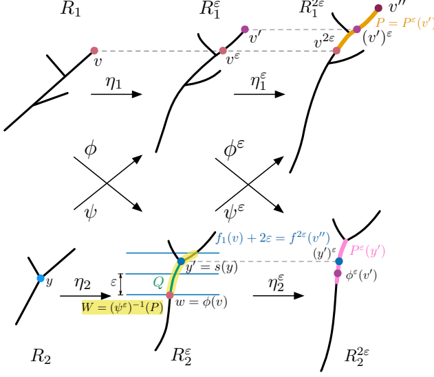
Fig. 5 An illustration for the proof of Theorem 1 .
