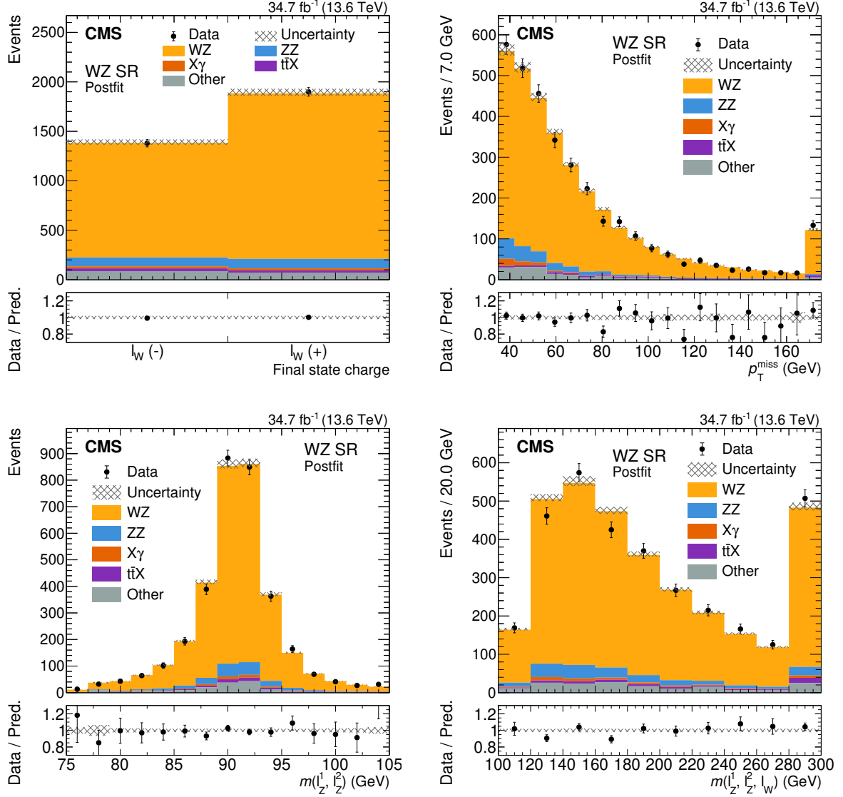
Figure 7. Distributions of several observables in the SR accounting for the fit to data. From upper left (sum of charge of the final-state leptons), upper right (missing transverse momentum), lower left (invariant mass of the two leptons assigned to the Z boson decay), and lower right (invariant mass of the triplepton system). The hatched band includes all systematic uncertainties. When present, overflow events are included in the last bin of the observables. The ratio panels show the ratio between data (black markers) with respect to the total prediction after the fit to data. Processes with a small contribution to this region are grouped in the “Other” category.
