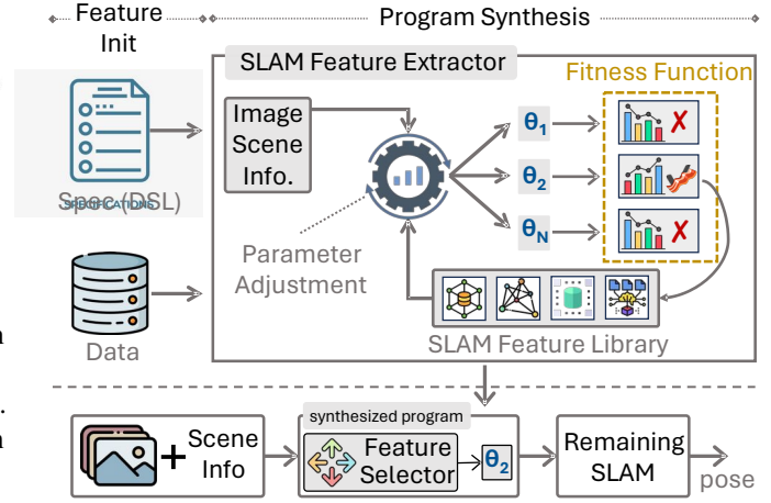
Fig. 2: A high-level overview of our approach.
