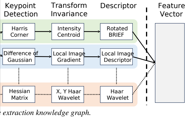
Fig. 7: Feature extraction knowledge graph.
