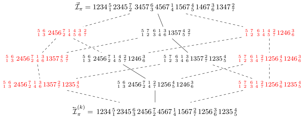
FIGURE 4. The \leq_\circ lower order ideal of \pi = 5761432 , a permutation of type (4, 7) . For each \iota \leq_\circ \pi , the Grassmannlike unit necklaces \mathcal{S}_{\bullet, \iota, \pi} is displayed (to save space, elements of \vec{\mathcal{I}}_\pi are omitted from intermediate necklaces). The weakly separated necklaces, which have insertion permutation \iota \in \text{Sep}_\pi , are in black. For example, any necklace containing 2456, 1347 is not weakly separated. Edges are cover relations in \leq_\circ : solid edges are edges in TG_\pi , while dashed edges are not. Since there is no solid path from the top to the bottom, \pi is not toggle-connected.
