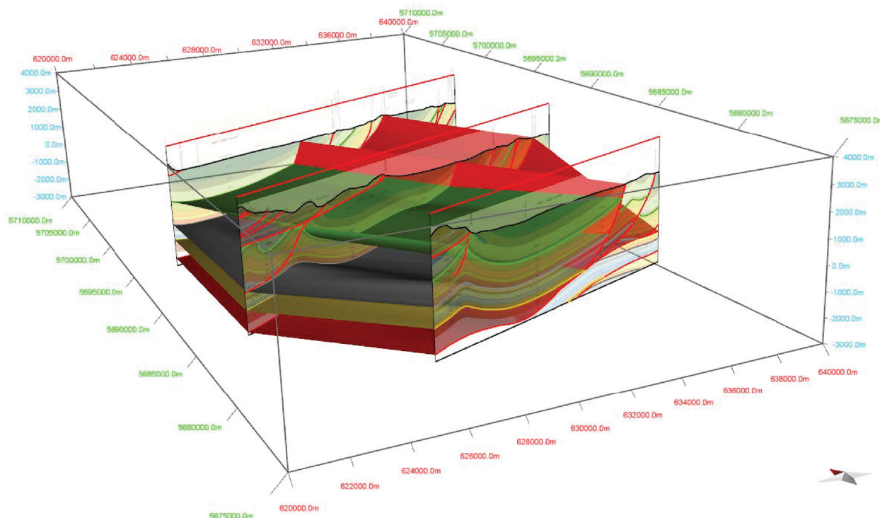
Figure 1. Completed 3D model of a fault system before restoration and validation. Figure modified from Petex (2022).
