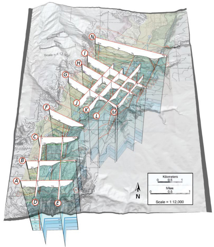
Figure 4. DEM with map overlay. Map features display surface observations. Cross sections (lettered) display subsurface fault and stratigraphic unit interactions. Fault and horizon surfaces were created by linking fault and horizon lines between sections.
