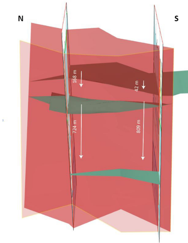
Figure 5. East-looking view between sections A and C. Faults A and B are partially transparent to show the displacement of the horizon between the Tenny Canyon Tongue (Jtc) and the Navajo Sandstone (Jn). Unit layers are dipping south, and fault A causes more displacement compared to fault B.
