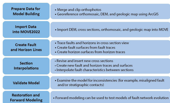
Figure 2. Six step modeling workflow used to develop the high-resolution 3D model of the Sevier fault zone.
