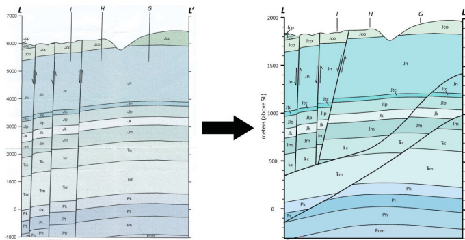
Figure 3. Cross-section prior to model building (left) vs. same cross-section revised after model building (right). Note especially the addition of two faults.
