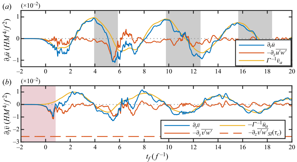
Figure 3. The horizontally averaged x- and y-momentum budget (4.1) at z = 3/4 for \Gamma = 10 . The red shaded region highlights the period when the dominant balance is described by SI-induced Reynolds stresses (red line) accelerating the mean along-front y-momentum (blue line). The linear SI mode transport at saturation is also shown. Following this ageostrophic perturbation, the front begins inertially oscillating. Grey shaded regions indicate periods when the Reynolds stress divergence damps the inertial oscillations (i.e. when \bar{u}_a > 0 coincident with -\partial_z \overline{u'w'} < 0 ).
