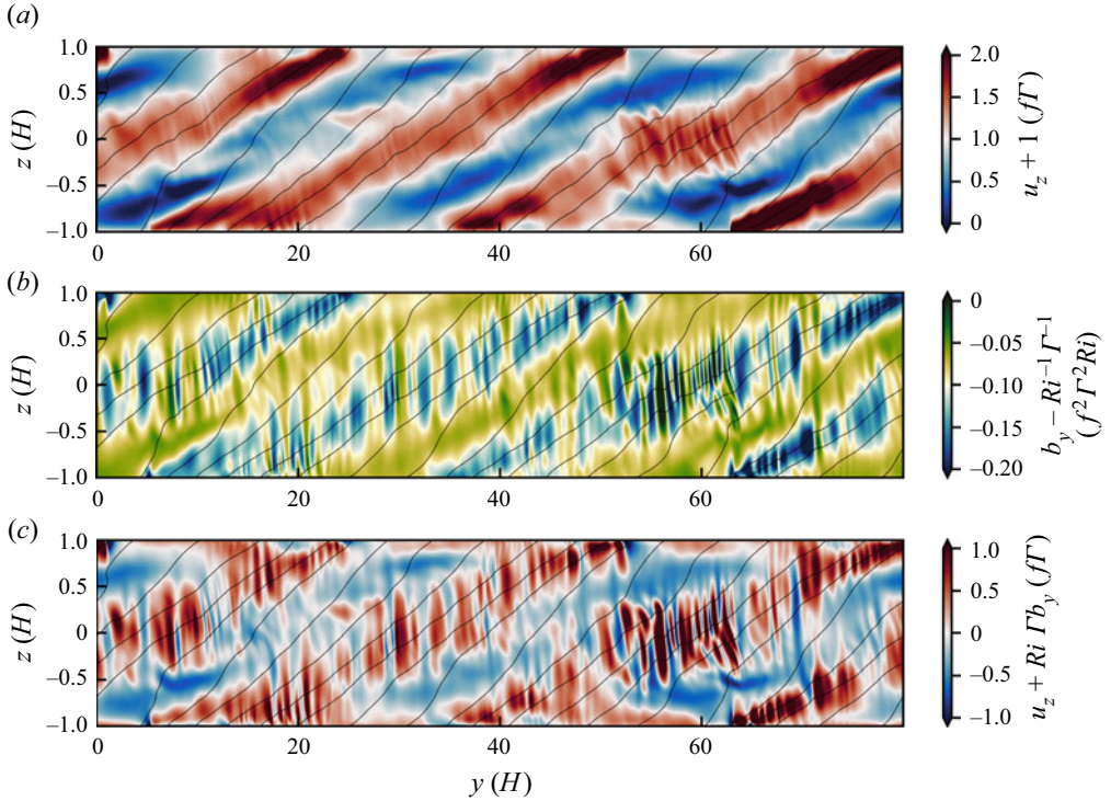
Figure 16. Sections of (a) the vertical derivative of the absolute momentum u_z + 1 , (b) the horizontal derivative of the total buoyancy b_y - Ri^{-1} \Gamma^{-1} , and (c) the thermal wind imbalance u_z + Ri \Gamma b_y from SIM18 after 20 inertial periods. Contours of total buoyancy are overlaid in black.
