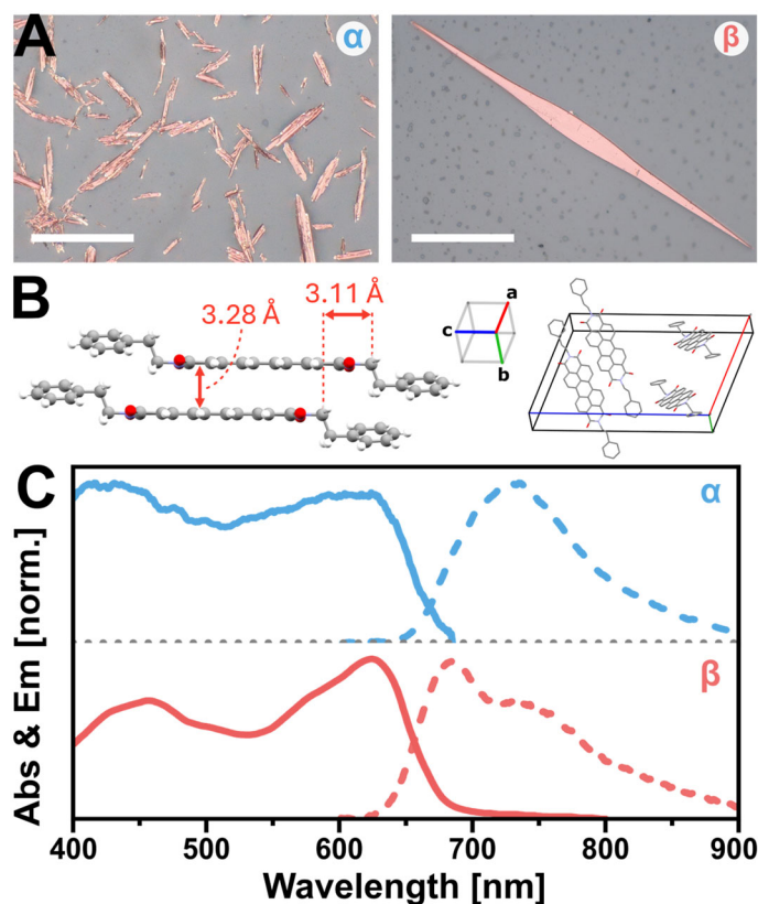
Figure 2: (A) Optical microscopy images of \alpha (left) and \beta (right) EP-PDI crystals grown via drop-casting a heated EP-PDI toluene solution onto DI-water at 20 °C and 40 °C respectively. The scale bar in both images is 50 \mu\text{m} . (B) Structure of an EP-PDI \alpha -crystal showing its unit cell and slip-stacked packing arrangement of neighboring EP-PDI molecules, with displacements of 3.28 Å along their \pi - \pi stacking direction, 3.11 Å along their long (longitudinal) axis, and 0.62 Å along their short (transverse) axis (not shown). The \pi - \pi stacking occurs primarily along the crystalline b -axis. (C) Absorption and PL spectra of \alpha - and \beta -crystals collected via absorption and emission microscopy.
