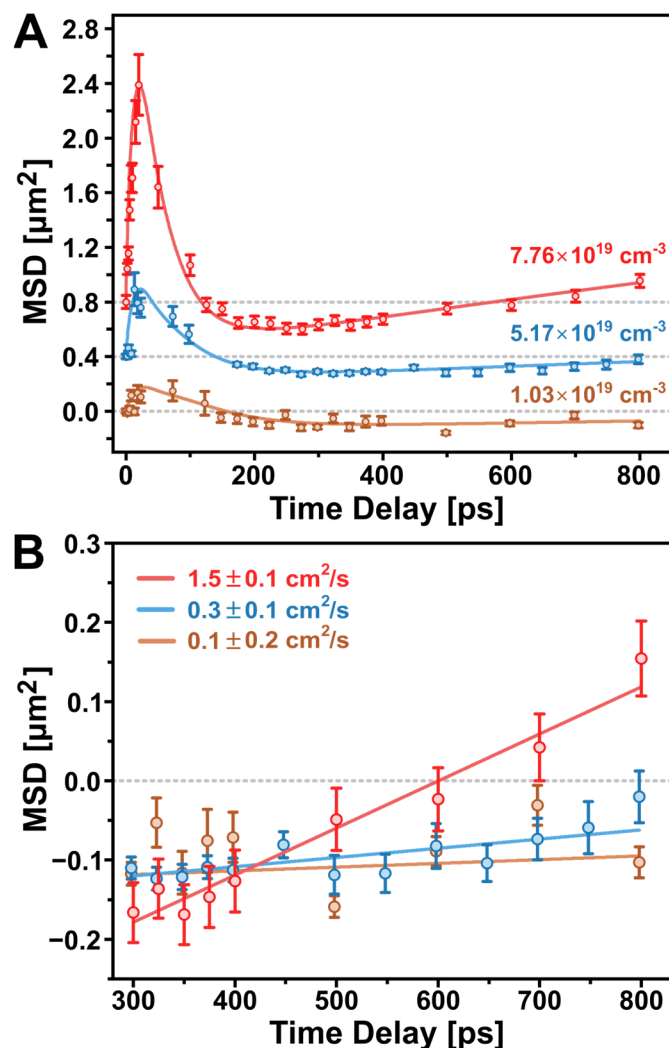
Figure 5: (A) MSD curves from three TAM diffusion measurements performed on an \alpha -crystal with varying excitation densities. The data are offset for clarity and gray dashed lines show the zero-point for each dataset. (B) Zoom in of the MSD curves at delays of 300 – 800 ps that highlight an increase in the MSD slope with increasing excitation density. The pump fluences used to collect the plotted data are 1893 \mu\text{J}/\text{cm}^2 (red), 1262 \mu\text{J}/\text{cm}^2 (blue), and 252 \mu\text{J}/\text{cm}^2 (brown).
