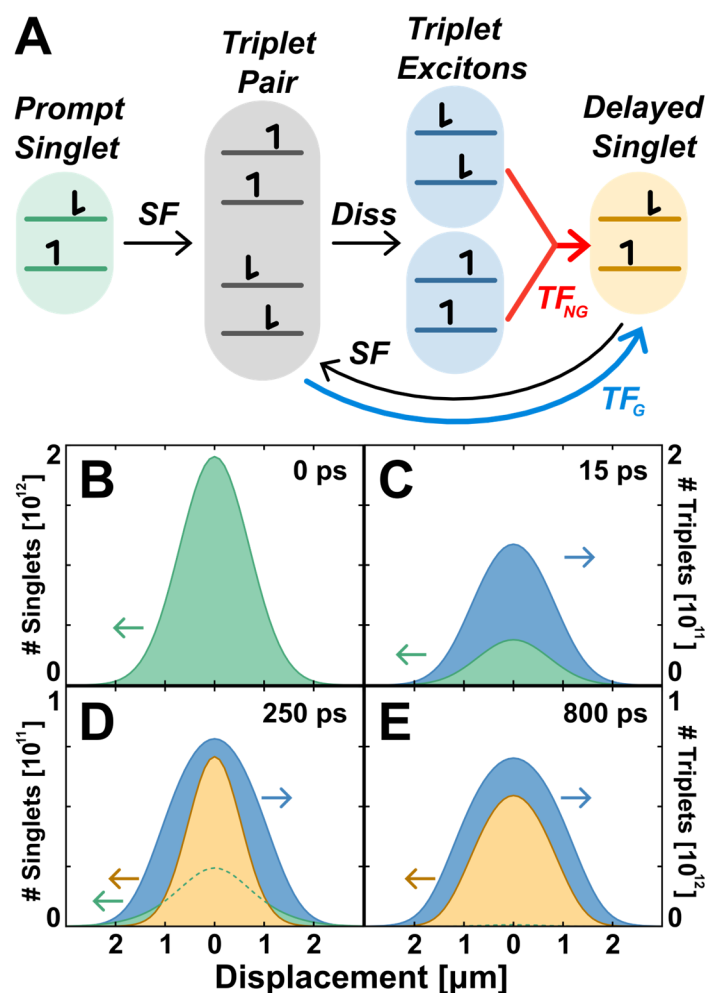
Figure 4: (A) Modified kinetic model for simulating the evolution of prompt singlets initially generated by the pump pulse and delayed singlets formed through geminate ( TF_G ) and non-geminate TF ( TF_{NG} ). (B–E) Profile slices of the simulated prompt singlet (green), triplet (blue), and delayed singlet (yellow) exciton distributions at four time points matching those highlighted in Figure 3A . Scales on the y-axes show the number of singlet (left) and triplet (right) excitons.
