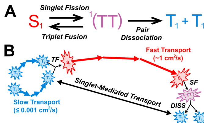
Figure 1: (A) Reaction scheme describing triplet pair, ^1(TT) , formation via singlet fission followed by either triplet pair dissociation into independent triplets, T_1 + T_1 , or triplet fusion to reform the singlet state, S_1 . (B) The interconversion of singlet and triplet populations via singlet fission and triplet fusion allows for singlet-mediated transport. Abbreviations: TF – triplet fusion; SF – singlet fission; Diss: Pair Dissociation.
