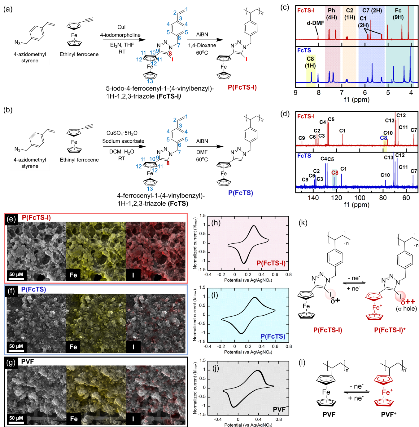
Figure 1. Synthesis of redox-active materials. Synthesis of redox-active (a) halogen bonding donor ( FcTS-I ) and (b) hydrogen bonding donor ( FcTS ) and their polymer. (c) ^1\text{H} NMR ( \text{C}_3\text{D}_7\text{NO} , 500 MHz) and (d) ^{13}\text{C} NMR ( \text{C}_3\text{D}_7\text{NO} , 125 MHz) spectra of FcTS-I and FcTS . High-resolution SEM images and EDS mapping of (e) P(FcTS-I) , (f) P(FcTS) , and (g) PVF electrodes. Twenty cycles of cyclic voltammograms of (h) P(FcTS-I) , (i) P(FcTS) , and (j) PVF electrodes in 100 mM TBAPF 6 at a scan rate of 30 mV/s in acetonitrile with activated carbon clothes as a counter and Ag/AgNO 3 as a reference electrode. CV plot was normalized by the peak oxidation current ( I/I_{\text{max}} ). Electrochemical responses of (k) P(FcTS-I) redox reaction and creation of the sigma hole and (l) PVF redox reaction.
