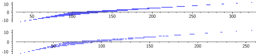
Fig. 1 For q = 11 and q = 9 , respectively, the graph shows all the points (\#A(\mathbb{F}_q), c_1) , where A ranges over abelian surfaces over \mathbb{F}_q , and c_1 = G^{[n-1]} = f_A^{[2n-1]} with n = 2 ; see (17)
