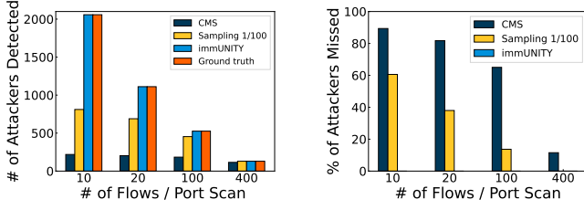
(a) Accuracy of detecting attackers (b) Inefficiency in detecting attackers Fig. 3: MAWI: port scan detection
