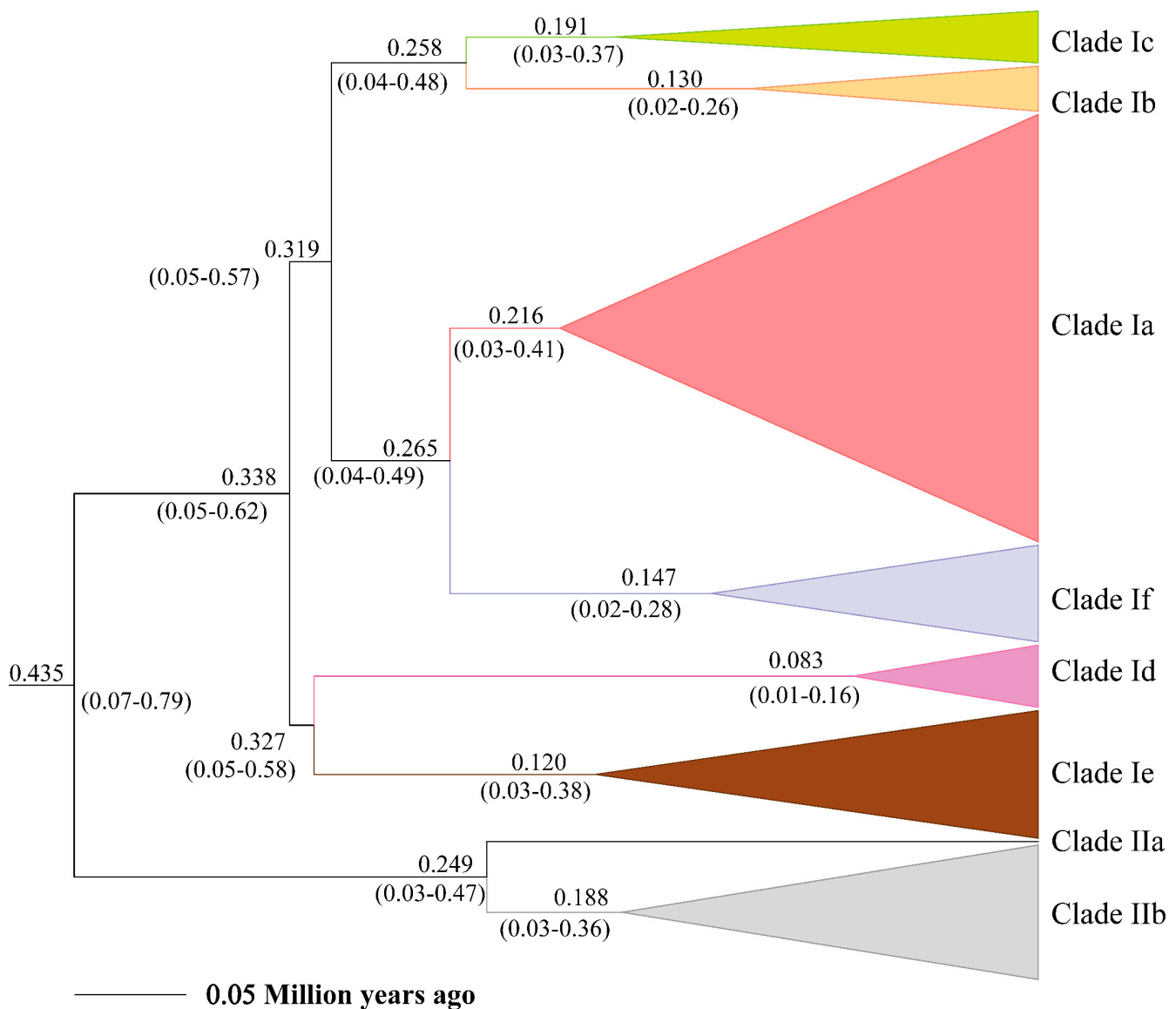
Figure 3. Estimate of divergence time of major lineages within Eremias argus derived from mtDNA cyt b data.
