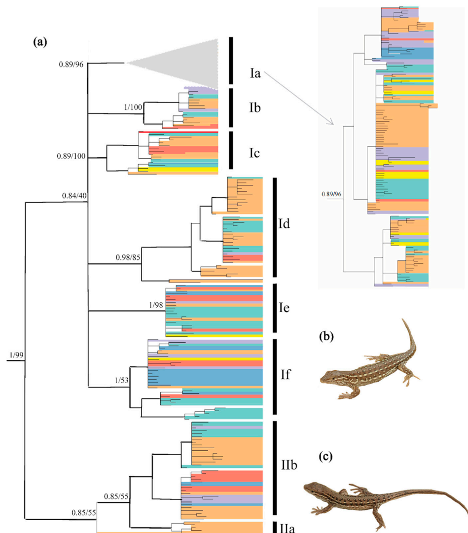
Figure 2. (a) Hypothesized phylogenetic relationships of Eremias argus included in this study, illustrated by the 50% majority-rule consensus tree resulting from partitioned Bayesian analyses. Bayesian posterior probabilities and maximum likelihood bootstrap values are shown. Distribution of the haplotype group across the species range refers to Figure 1; (b) Eremias argus with eye-like dorsal pattern; (c) Eremias argus with a striped dorsal pattern. Photos by X.G. (b,c) show two morphotypes of Eremias argus , and their reciprocal monophyly is rejected in the phylogenetic tree.
