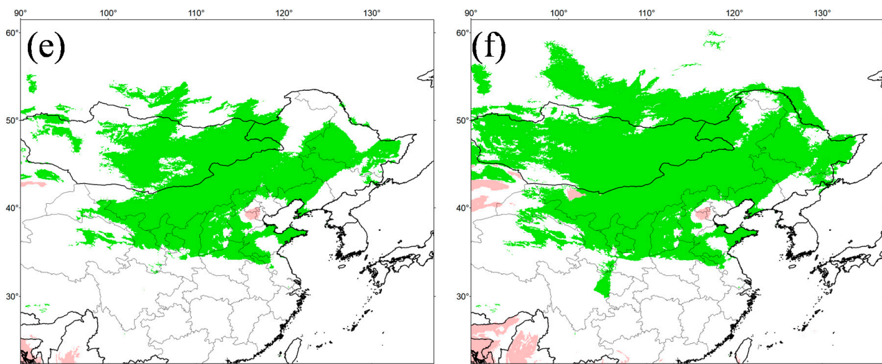
Figure 8. Potentially suitable distribution area in six different periods for Eremias argus . (a) MPWP, Mid-Pliocene Warm Period; (b) MIS 19, Marine Isotope Stage 19; (c) LIG, Last Interglacial (d) LGM, Last Glacial Maximum; (e) SSP 126 for 2070s, Shared Socio-economic Pathway 126; (f) SSP 585, Shared Socio-economic Pathway 585 for 2070s. (a,b) show the separate projections for MPWP and MIS 19 by running the model in current times with the variables in Paleoclim. (c–f) show the separate projections for LIG, LGM, SSP 126 and SSP 585 by running the model in current times with the variables in Wordclim. Negative MESS scores, shown as similarity <0 by pink, indicate areas without current equivalents of climatic conditions.
