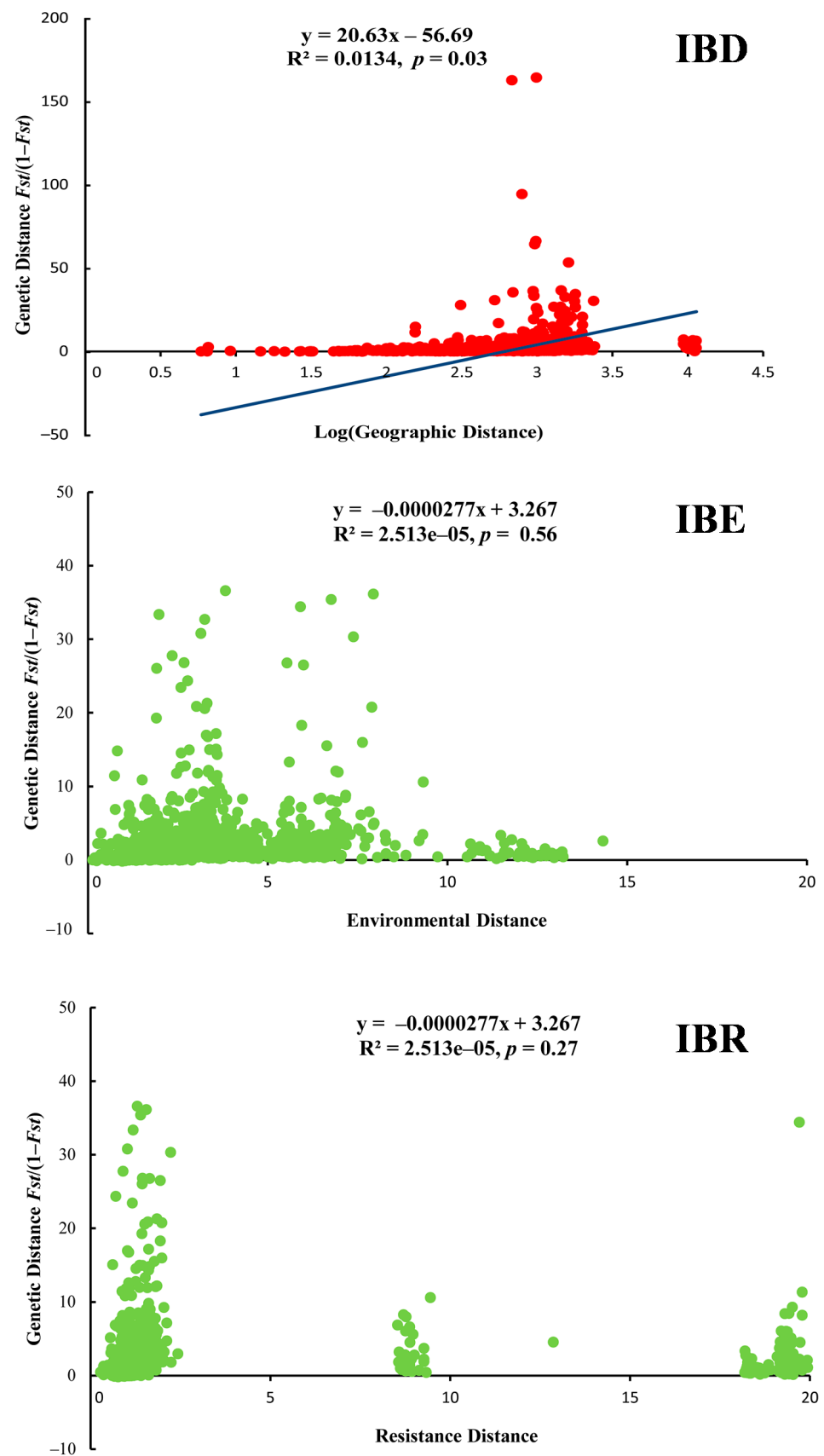
Figure 4. Correlations between genetic, environmental, geographic distances and resistance (IBD, IBE and IBR analysis results of Eremias argus ).
