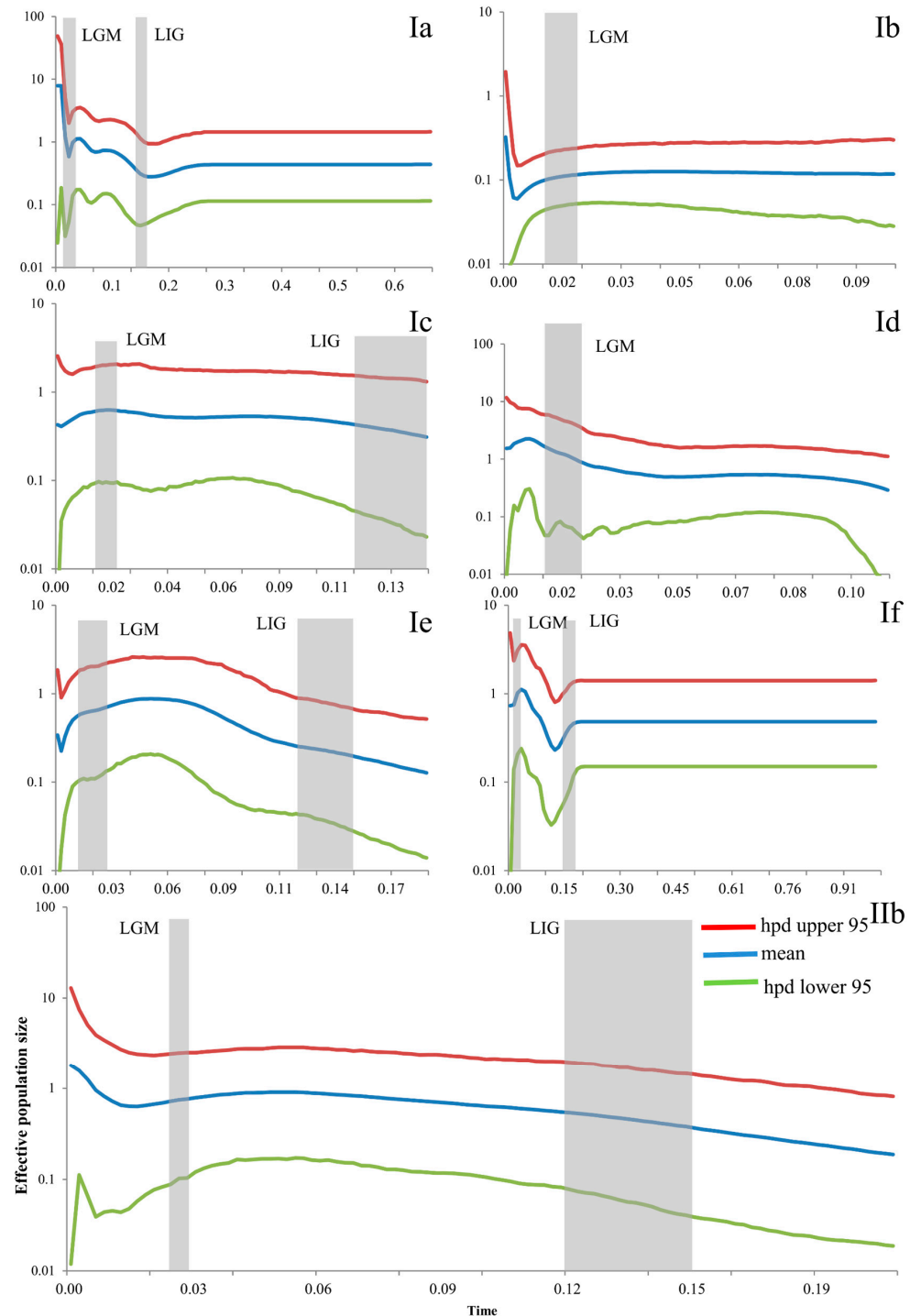
Figure 6. Bayesian skyline plots (BSP) of the seven subclades for Eremias argus . The y-axes represent the estimated effective population size on a log scale ( Ne \times \tau / 10^6 , the product of the female effective population size and generation length in years); x-axes represent time in millions of years ago (Ma). Vertical dark-grey bars represent the duration of the Last Glacial Maximum (LGM), or the Last Interglacial (LIG). Ia–IIb refers to the clade recovered in Figure 2.
