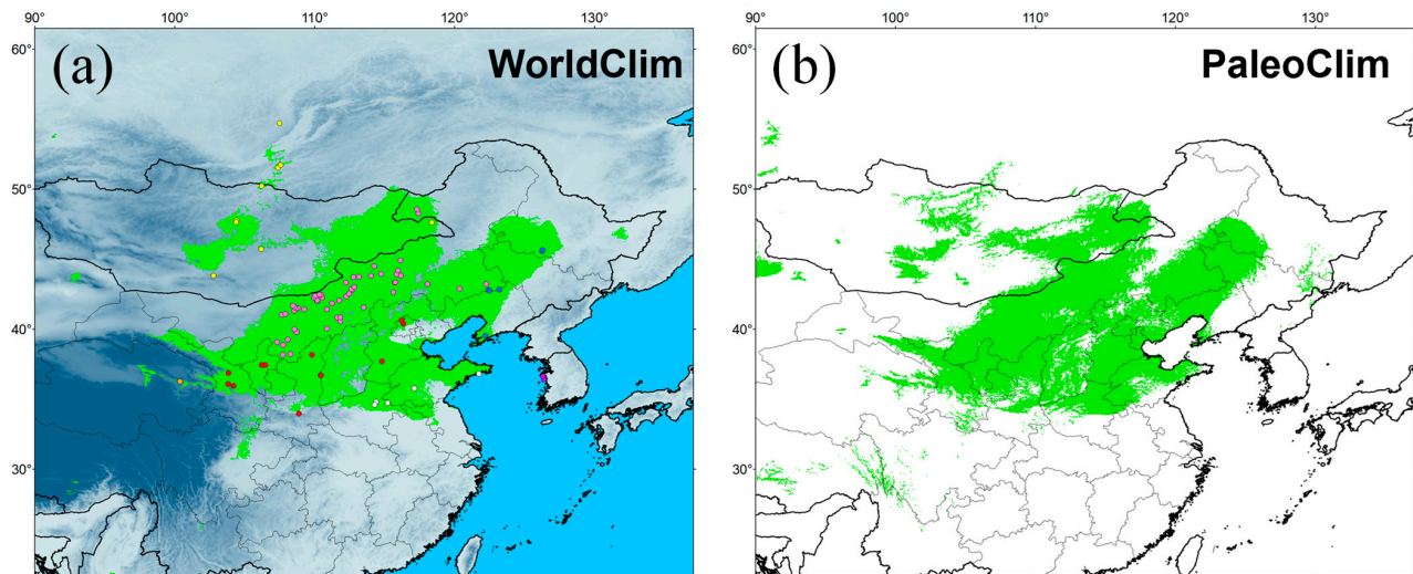
Figure 7. Potentially suitable distribution area obtained with MaxEnt for Eremias argus at present. Green indicates highly suitable habitat area. Climate variables are from WorldClim (a) and PaleoClim (b).
