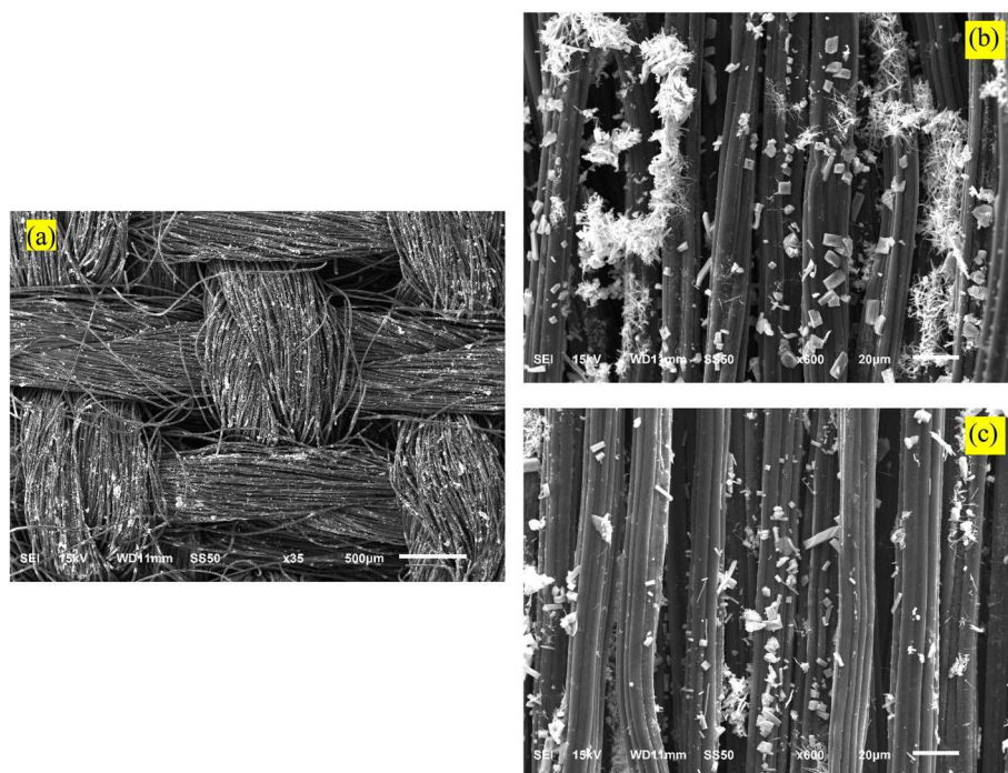
Fig. 2 SEM images of \text{Ru}_{0.75}\text{Pt}_{0.25}/\text{ACC} . (a) Magnification: 35\times reveals dispersal of the noble metal particles and (b) and (c) magnification: 600\times reveals morphology of noble metal particles.
