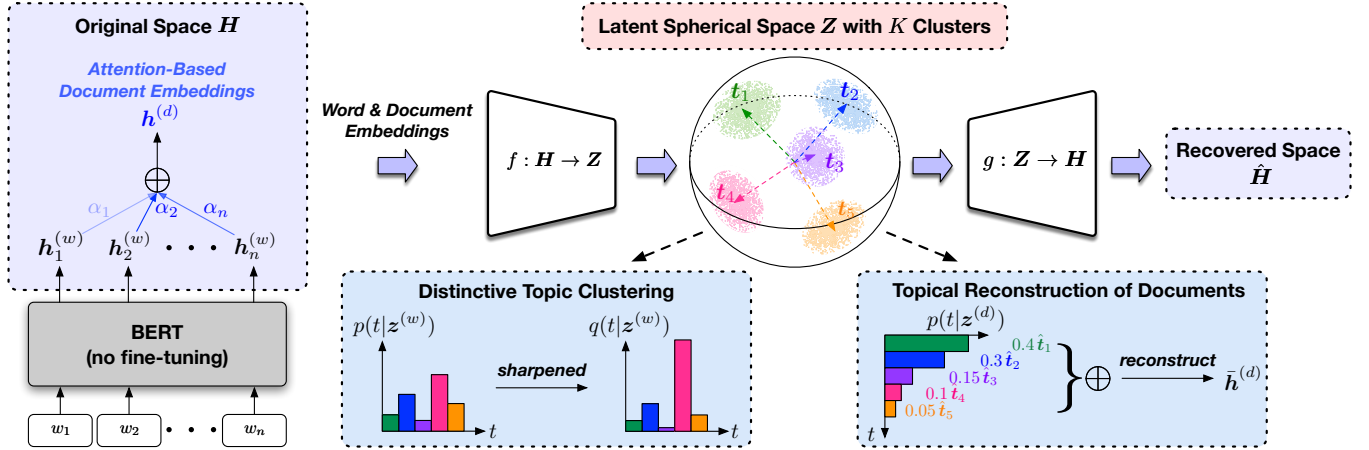
Figure 2: Overview of TopClus. We assume that the K -topic structure exists in a latent spherical space Z . We jointly learn the attention weights for document embeddings and the latent space generation model via three objectives: (1) a clustering loss that encourages distinctive topic learning in the latent space, (2) a topical reconstruction loss of documents that promotes meaningful topic representations for summarizing document semantics and (3) an embedding space preserving loss that maintains the semantics of the original embedding space. The PLM is not fine-tuned.
