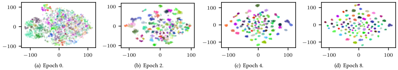
Figure 4: Visualization using t-SNE of 3,000 randomly sampled latent word embeddings during training. Embeddings assigned to the same cluster are in the same color. The latent space gradually exhibits distinctive and balanced cluster structure.
