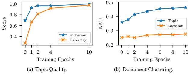
Figure 5: Study of TopClus training on NYT. We show (a) topic coherence measured by intrusion test and topic diversity and (b) document clustering NMI scores over training.
