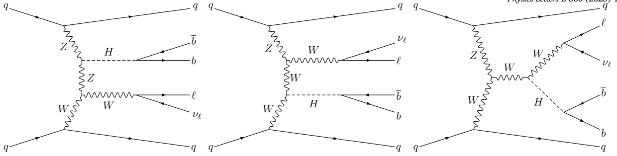
Fig. 1. Tree-level Feynman diagrams for the production of WH \rightarrow \ell \nu b \bar{b} via VBS, where \ell is an electron or muon.
