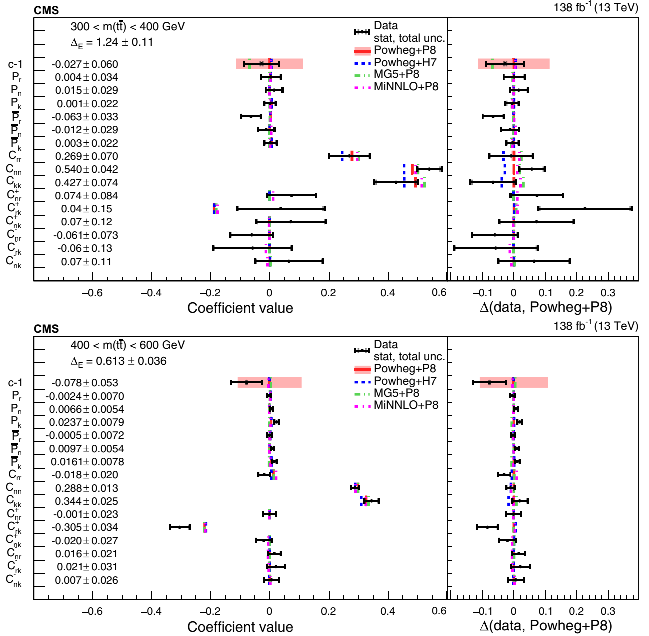
FIG. 19. Results of the full matrix measurement in bins of m(\bar{t}\bar{t}) . The measurements (markers) are shown with the statistical uncertainty (inner error bars) and total uncertainty (outer error bars) and compared to the predictions of POWHEG+PYTHIA, POWHEG+Herwig, MadGraph5_aMC@NLO+PYTHIA and MiNNLO+PYTHIA. In the right panels, results are presented with the POWHEG+PYTHIA predictions subtracted. The POWHEG+PYTHIA prediction is displayed with ME scale and PDF uncertainties. The values of \Delta_E are displayed for each measurement.
