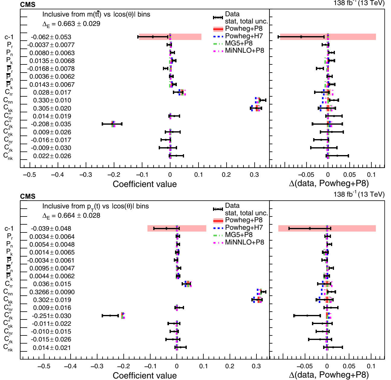
FIG. 17. Results of the inclusive full matrix measurement obtained by combining the bins of the m(t\bar{t}) vs |\cos(\theta)| (upper) and p_T(t) vs |\cos(\theta)| (lower) measurements. The measurements (markers) are shown with the statistical uncertainty (inner error bars) and total uncertainty (outer error bars) and compared to the predictions of POWHEG+PYTHIA, POWHEG+Herwig, MadGraph5_aMC@NLO+PYTHIA and MiNNLO+PYTHIA. In the right panels, results are presented with the POWHEG+PYTHIA predictions subtracted. The POWHEG+PYTHIA prediction is displayed with ME scale and PDF uncertainties. The values of \Delta_E are displayed for each measurement.
