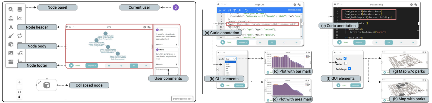
Fig. 3: Left: Main elements of Curio's interface. Center, Right: Connecting facets from the same node. Center: A drop-down menu listing mark attributes is created through an annotation in a Vega-Lite specification. Right: A checkbox is created, but now through an annotation in Python code.
