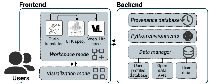
Fig. 4: Curio's frontend and backend components.
