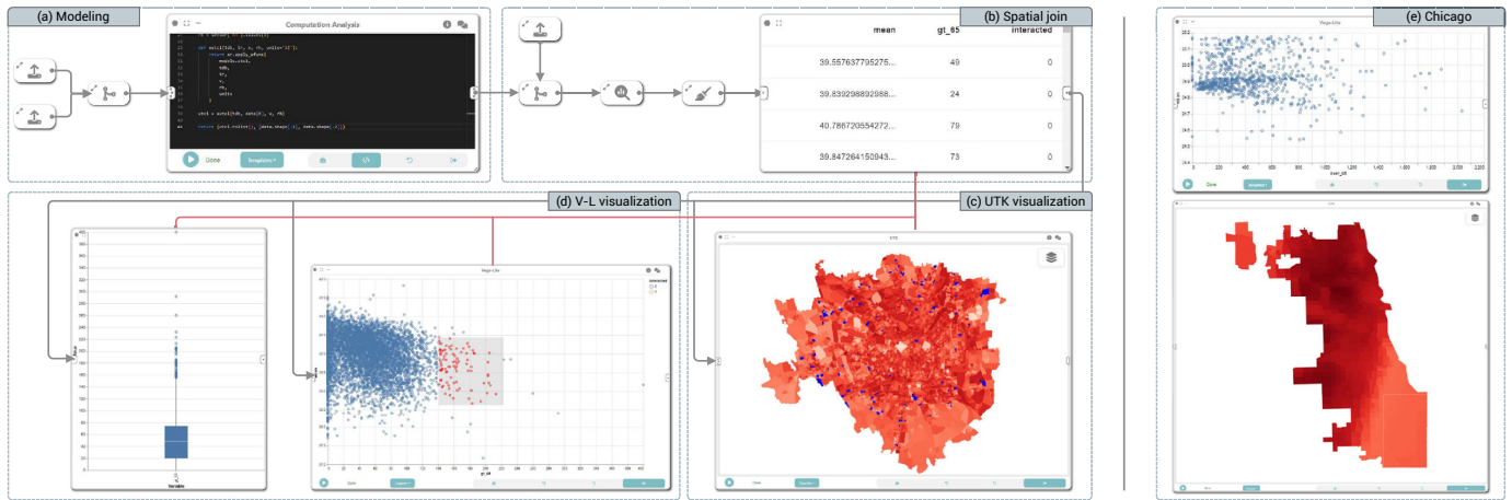
Fig. 6: Using Curio to create visualizations leveraging multiple datasets. (a) The user loads weather data and computes the UTCL, (b) followed by a spatial join with a physical layer describing neighborhoods in Milan. (c,d) The user then creates linked visualizations that highlight neighborhoods with high UTCL and a large population of older adults. (e) By changing two nodes, the user can create a similar visualization using data from Chicago.
