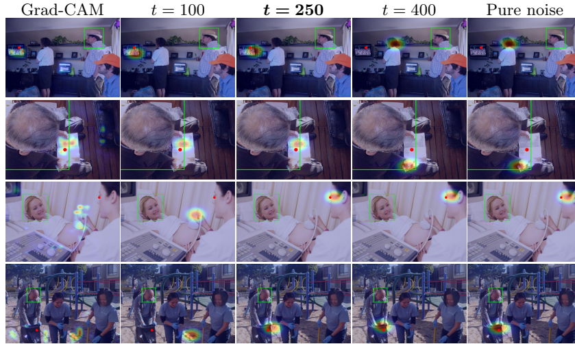
Fig. 5: Diffusion model output for noise added at different timesteps. Red dots represent the ground truth annotation. Adding noise at earlier steps generates outputs on high Grad-CAM response regions. Adding noise at later steps generates outputs similar to sampling from pure noise. Noise at step 250 is the best trade-off.
