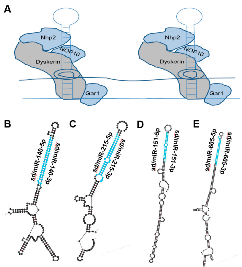
Figure 3. miRNAs derived from Box H/ACA snoRNA-like transcripts that bind dyskerin. (A) Schematic of box H/ACA snoRNP bound to dyskerin complex, giving rise to snoRNP. Dyskerin complex includes Dyskerin, NHP2, NOP10, and GAR1 [18]. (B–E) Most thermodynamically stable secondary structures of box H/ACA snoRNA-like transcripts known to bind dyskerin complex [40] were generated by mfold [20]. Mature miRNA sequences derived from these transcripts are highlighted in blue. (B) Box H/ACA snoRNA-like transcript (GRCh38: chr 16:69933072-69933264:1) was identified to bind dyskerin and encompasses miR-140 (ENSG00000208017) which functions as a tumor-suppressing RNA and is downregulated in prostate cancer [41]. (C) Box H/ACA snoRNA-like transcript (GRCh38: chr1:220117845-220118007:-1) was identified to bind dyskerin and surrounds miR-215 (ENSG00000207590) which is known to function as a tumor suppressor and is downregulated in ovarian, colorectal, prostate and lung cancer [42,43]. (D) Box H/ACA snoRNA-like transcript (GRCh38: chr8:140732552-140732807:-1) was determined to bind dyskerin and encapsulates miR-151 (ENSG00000254324) which is recognized as a tumor-suppressing RNA and is downregulated in prostate cancer [44–46]. (E) Box H/ACA snoRNA-like transcript (GRCh38: chr 10:51299393-51299708:1) was determined to bind dyskerin and surrounds miR-605 (ENSG00000207813) which is described to act as a tumor-suppressing RNA in melanoma, colorectal, breast, lung and prostate cancer [47–51].
