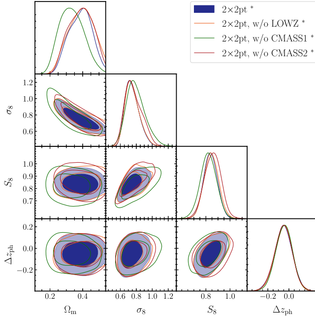
FIG. 12. Cosmological constraints with 2 \times 2 pt but removing a single lens redshift bin from each analysis.
