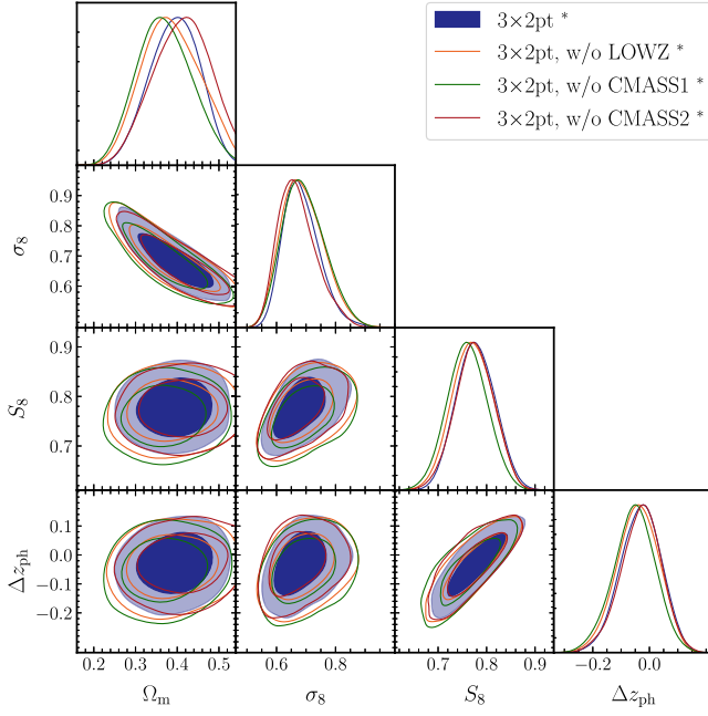
FIG. 11. Cosmological constraints with 3 \times 2 pt but removing a single lens redshift bin from each analysis.
