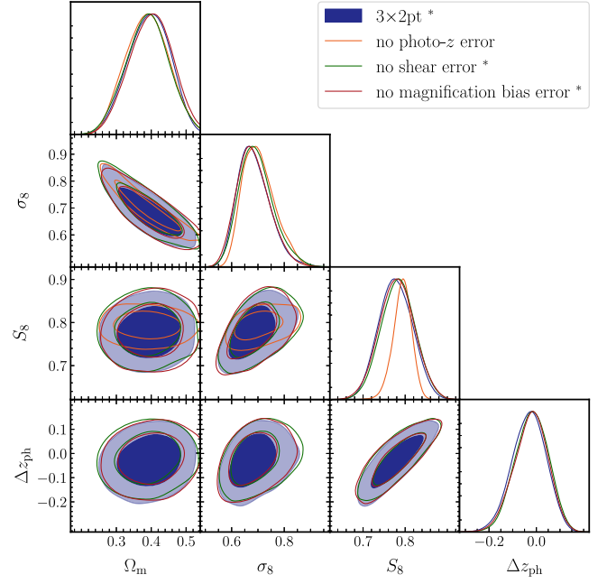
FIG. 13. Cosmological constraints with 3 \times 2 pt but fixing one of the nuisance parameters to zero.
