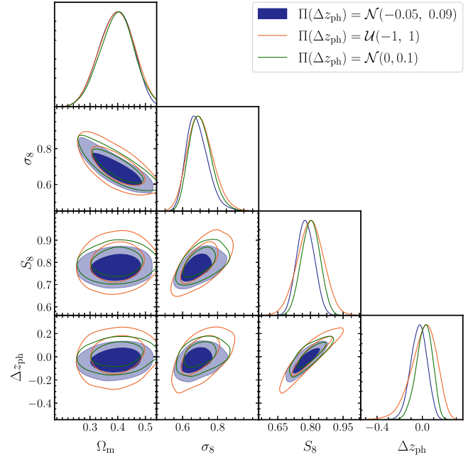
FIG. 3. Cosmological parameter constraints for HSC-Y3 3 \times 2 pt analyses with three different \Delta z_{\text{ph}} prior choices; the informative prior taken from the fiducial small-scale analysis result, the uninformative prior \mathcal{U}(-1, 1) , and the informative prior \Pi(\Delta z_{\text{ph}}) = \mathcal{N}(0, 0.1) .
