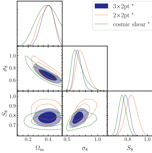
FIG. 2. The cosmological parameter constraints for the baseline 3 \times 2 pt, 2 \times 2 pt, and cosmic shear analyses. Here, every analysis uses the informative prior on \Delta z_{\text{ph}} from the HSC-Y3 small-scale analysis by Miyatake et al. [16].
