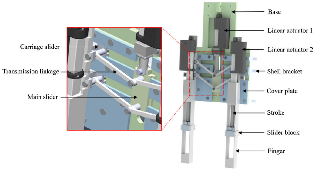
Figure 2. 3D model of the variable stiffness gripper.
