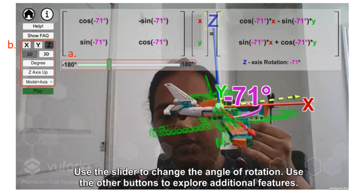
Fig. 1. Workshop 1: Virtual Model Rotation. (a) Slider for rotation (b) UI elements to visualize 2D vs 3D, radian vs degree, Z-axis up vs Z-axis down.
