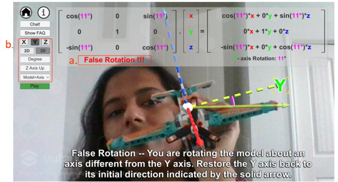
Fig. 2. Workshop 2: Physical Model Rotation (a) False rotation flag (b) UI elements to visualize 2D vs 3D, radian vs degree, Z-axis up vs Z-axis down.
