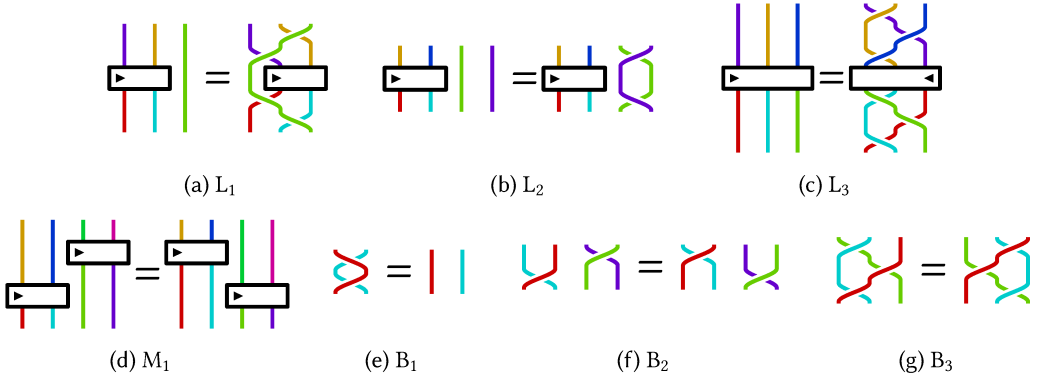
Fig. 5. Diagrammatic equivalence rules. The L_1 , L_2 , and L_3 moves correspond to our first step LAYER , M_1 corresponds to SWAP , and B_1 , B_2 , B_3 correspond to BRAID . Our canonicalization algorithm rewrites two words X_1, X_2 to a shared canonical form if and only if they can be rewritten into each other with these seven moves.
