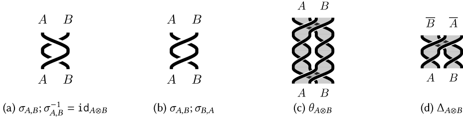
Fig. 6. Various morphisms in braided (6a, 6b), balanced (6c), and twisted involutive monoidal categories (6d).
