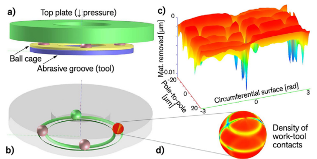
Fig. 33. BEAST simulation of ceramic ball-grinding [171].
