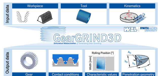
Fig. 30. Configuration of the GearGRIND3D simulation.
