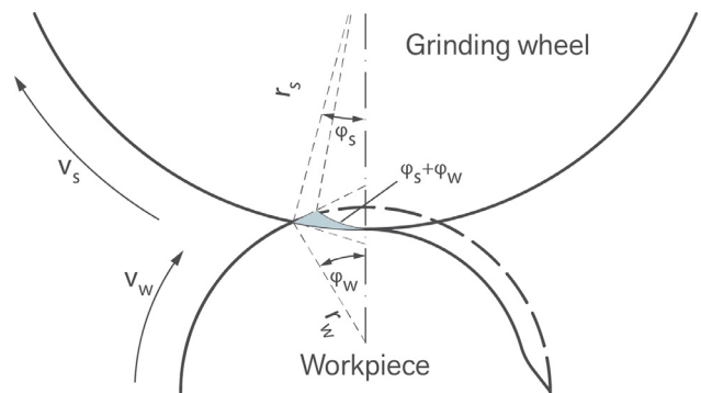
Fig. 2. Geometry and kinematics of cylindrical OD grinding according to Alden (adapted from [7]).
