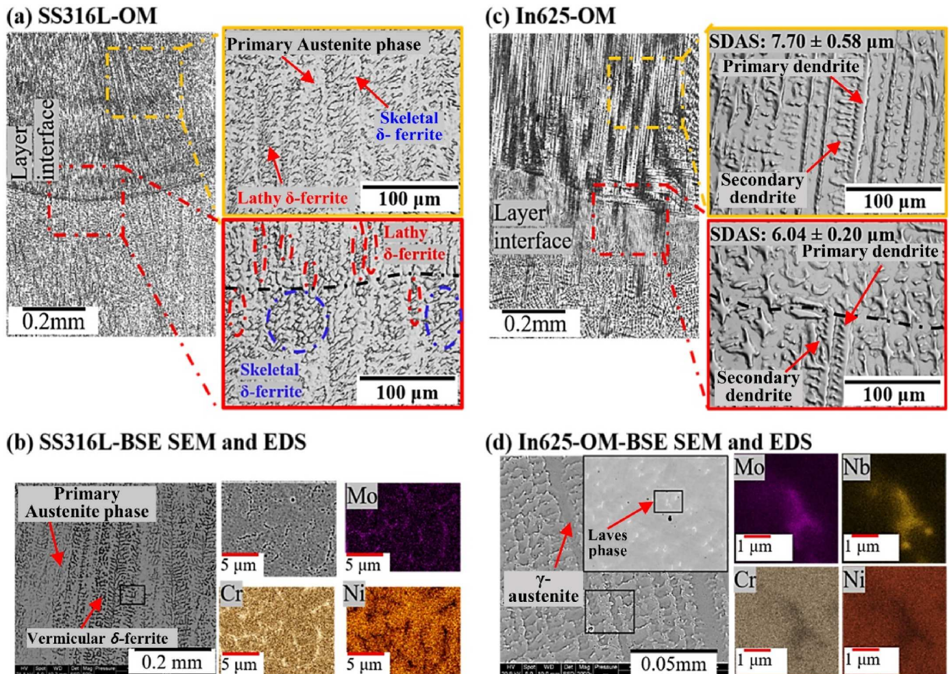
Fig. 4. Microstructure and compositional results from OM and SEM analysis on (a–b) SS316L and (c–d) In625 sides.
