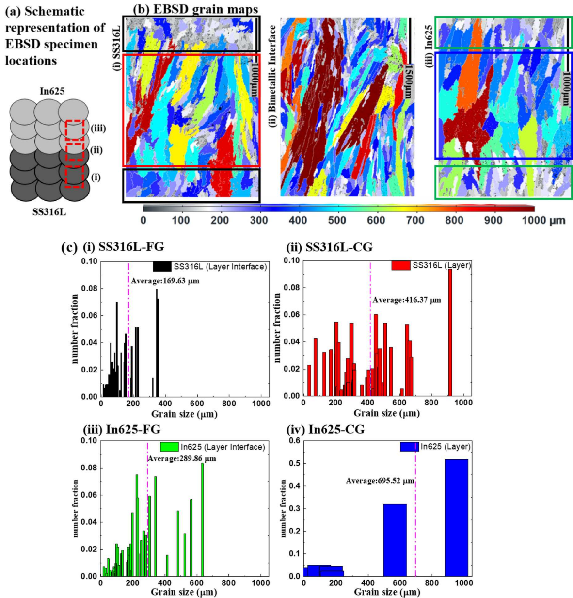
Fig. 7. (a) Schematic representation of EBSD analysis locations; (b) EBSD grain maps for (i) SS316L, (ii) bimetallic interface, and (iii) In625; (c) Location-specific grain size distribution on the (i) SS316L- FG, (ii) SS316L- CG, (iii) In625- FG, and (iv) In625- CG.
