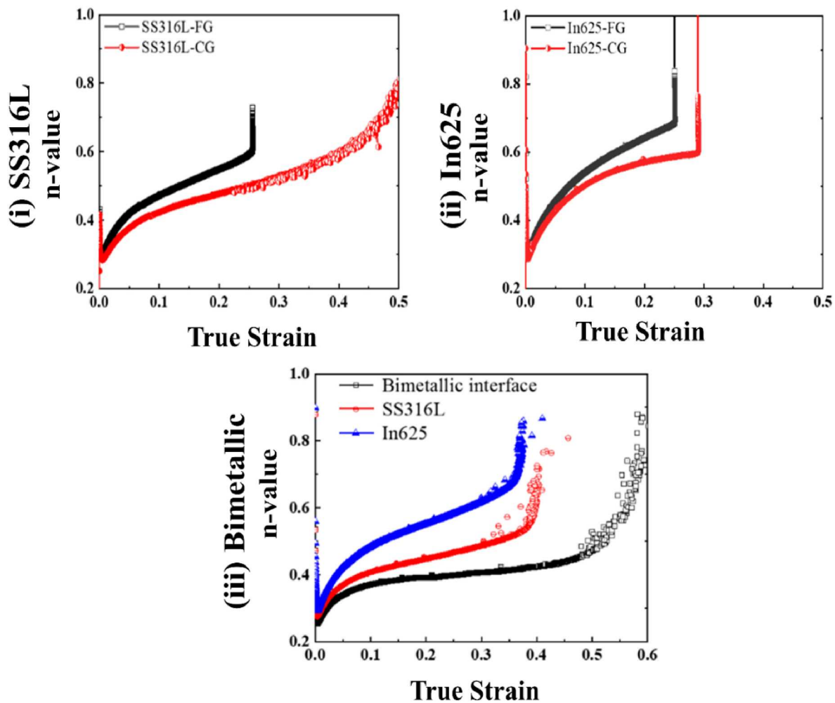
Fig. 11. Calculated n -value on the marked locations in Fig. 10 for (i) SS316L, (ii) In625, and (iii) bimetallic specimens.
