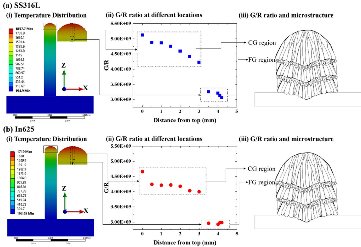
Fig. 13. (i) Thermal map, (ii) G/R ratio, and (iii) Schematic representation of the microstructure for (a) SS316L and (b) In625.
