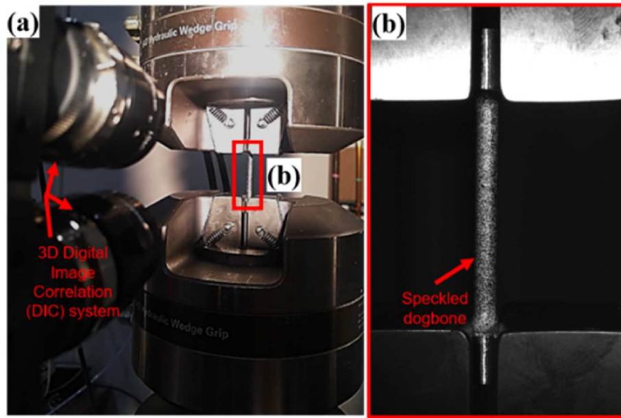
Fig. 2. (a) Experiment setup for digital image correlation (DIC) and (b) representative optical image of a dog-bone specimen with a black-on-white speckle pattern.
