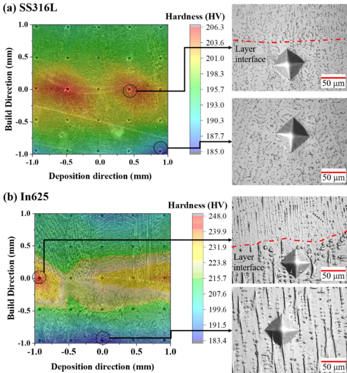
Fig. 12. Hardness data on the layer interfaces of (a) SS316L and (b) In625 are plotted as contour maps with micrographs of the highest and lowest hardness indents.
