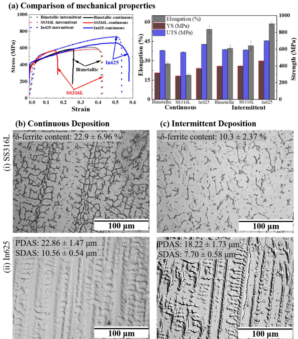
Fig. 16. Comparison of (a) mechanical properties and (b–c) microstructure between CDS and IDS.
