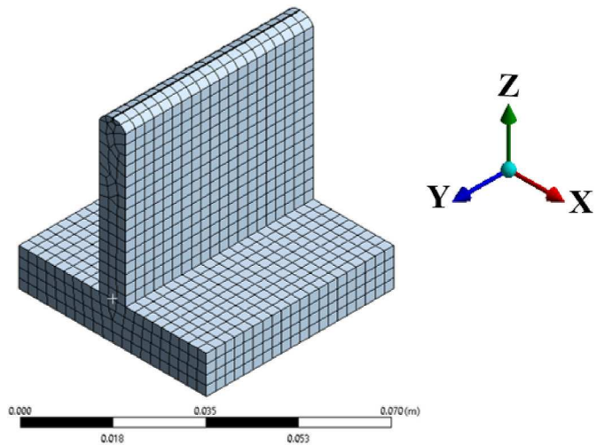
Fig. 3. FE model geometry with associated mesh.
