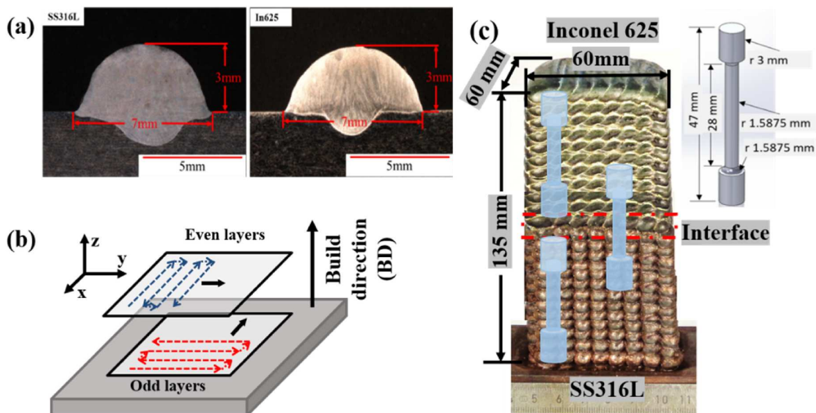
Fig. 1. (a) Bead cross-section on the yz plane with measurements from single-layer deposits of SS316L and In625 [9], (b) schematic representation of the arc movement [9], and (c) the fabricated bimetallic structure of SS316L and In625 with the dimensions and location of the tensile test specimens.
