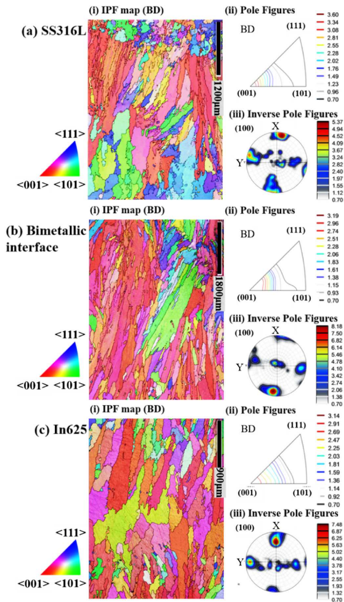
Fig. 6. (i) Inverse Pole figure (IPF) maps, (ii) Pole figure, and (iii) Inverse Pole Figures (IPFs) for (a) SS316L, (b) bimetallic interface, and (c) In625.
