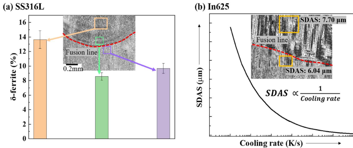
Fig. 14. (a) Location-specific ferrite content on SS316L and (b) SDAS vs. cooling rate graph reproduced from Ref. [48] with micrograph from a layer interface with SDAS value measured.
