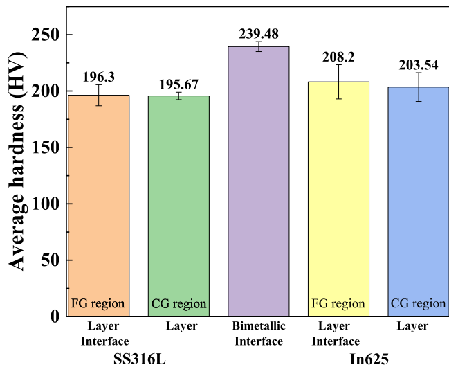
Fig. 8. Location-specific average hardness on the SS316L, bimetallic interface, and In625 sides.
