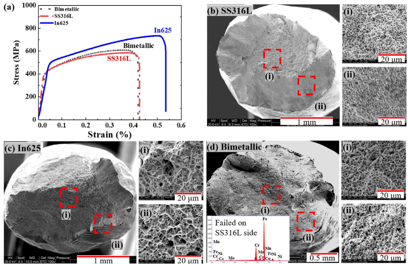
Fig. 9. (a) Stress vs. strain curves, (b–d) secondary electron SEM results from the fracture surface with a compositional analysis of the fracture surface of the bimetallic specimens inset of (d).
