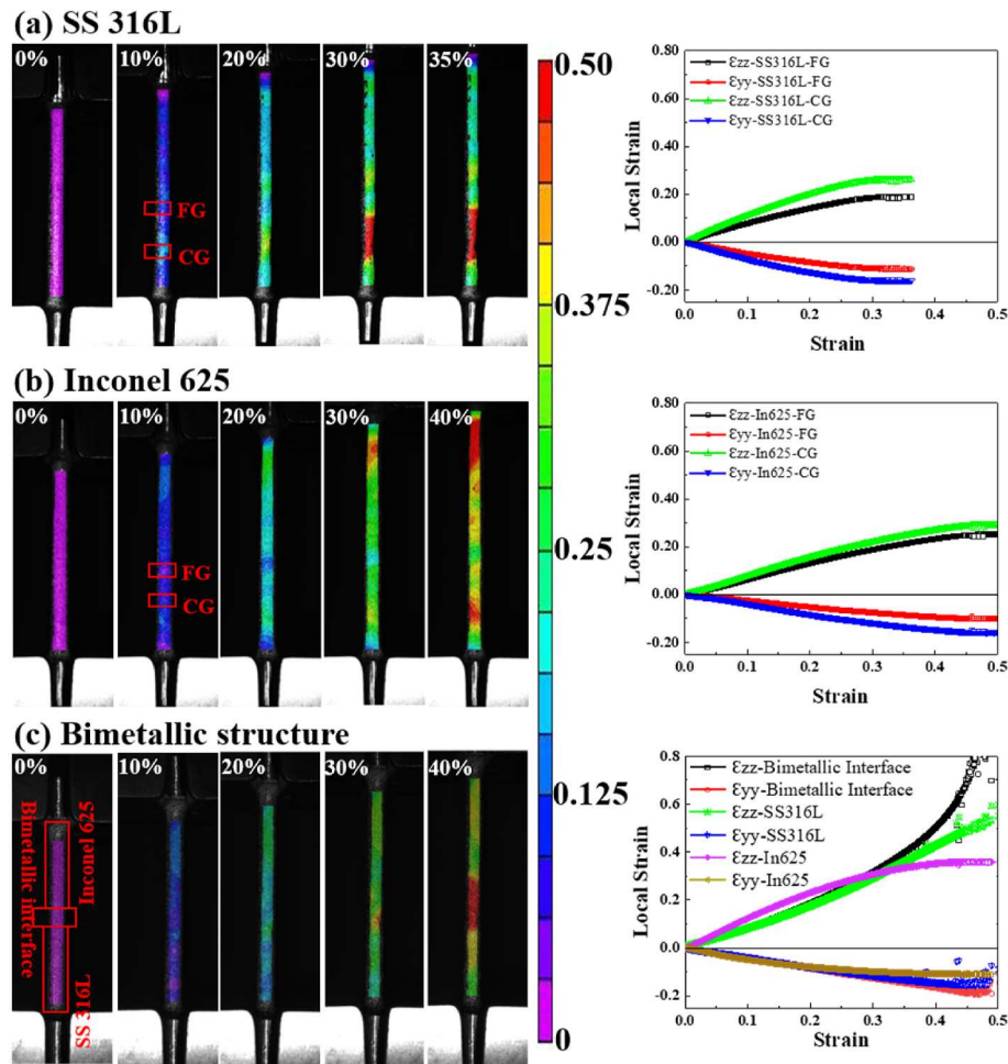
Fig. 10. 2D-strain maps at varying global strain values along with plots showing the evolution of the local strain as a function of total (i.e., global) strain for (a) SS316L, (b) In625, and (c) bimetallic specimens.
