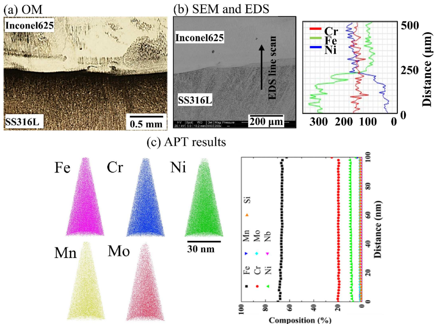
Fig. 5. Microstructure and compositional analysis results on the bimetallic interface from (a) OM, (b) SEM and EDS, and (c) APT.
