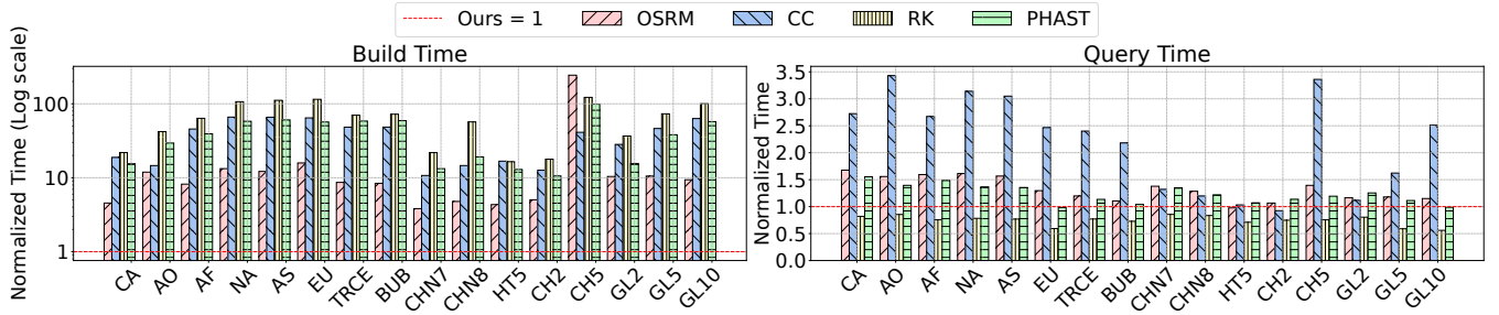
Figure 4: Build time and query time of all tested baselines, normalized to our algorithm. Lower is better. Since all running times are normalized to our algorithm, “Ours” is always equal to one, represented by the horizontal red dotted line.
