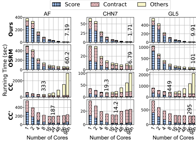
Figure 7: Running time of SPoCH (Ours), OSRM and CH-Constructor (CC) across different core counts. Lower is better. The fastest running time across all core counts is given above its bar. “96h”: 96 cores with hyper-threads. As the “Others” cost in CC dominates in most cases, we also report a version of CC that excludes this time, referred to as CC’.
