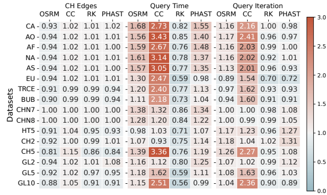
Figure 5: Heatmap of number of CH edges, query time, and query iteration. All numbers are normalized to ours. Blue or smaller is better.
