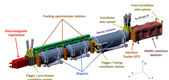
Figure 1. A sketch of the FASER detector, showing the different sub-detector system. The detector coordinate is also shown [2].
