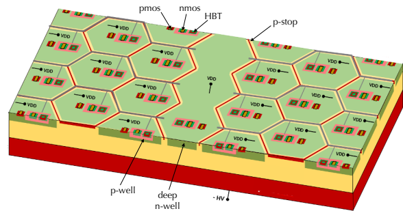
Figure 7. A sketch of the SiGe BiCMOS chip for the new FASER preshower [8].
