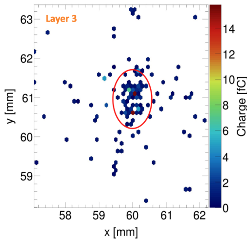
Figure 5. Charge distribution in the third layer of the detector from two electromagnetic showers initiated by 1 TeV photons with 500 \mu\text{m} separation.
