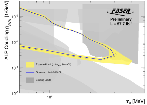
Figure 2. Interpretation of the signal region yield as ALP exclusion limits with the assumption of 0.42 neutrino background events. Systematic and statistical uncertainties described in Table 1 are included [4].
