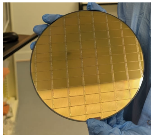
Figure 8. A post-processed wafer received in May 2024.
