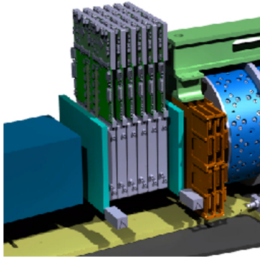
Figure 4. A sketch of the new preshower detector.
