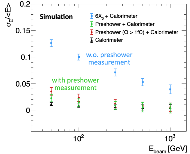
Figure 6. Energy resolution as a function of beam energy. The preshower detector does not degrade the performance of the energy measurement of the calorimeter with preshower correction for the energy above 100 GeV.
