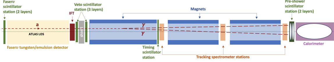
Figure 3: A typical ALP signal event traversing FASER. The neutral ALP (dotted line) enters the detector from the left.
