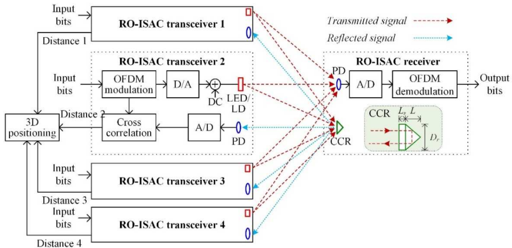
Fig. 1. Schematic diagram of a RO-ISAC system supporting 3D positioning.
