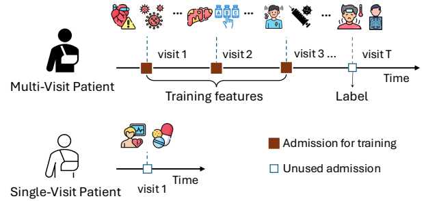
Figure 1. Example of supervised training on patient-level admission records in most predictive models
