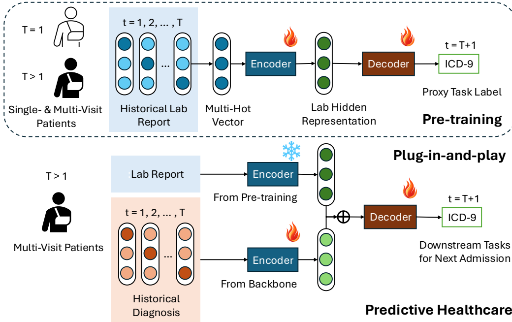
Figure 2. Overview of the proposed MPLite Framework
