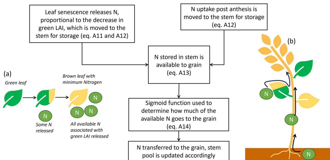
Figure A2. The allocation of N to the wheat grains post-anthesis, with equations indicated appropriately. Panel (a) is a visual representation of a leaf releasing N as the leaf area senesces. Panel (b) shows the three locations where N is transferred to the grain from post-anthesis N uptake, N stored in the stem, and senescing leaf area.
