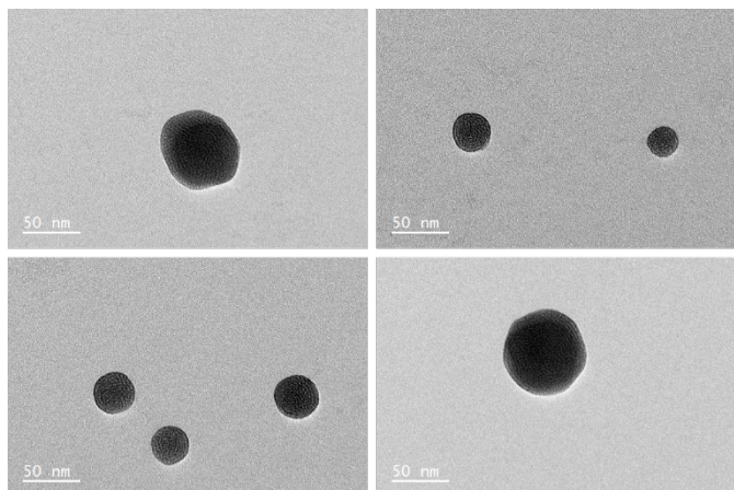
Figure 6. TEM images of a sample containing 0.05 mM CTAB and 0.1 mM POM1 , revealing the formation of CTAB- POM1 vesicles.
