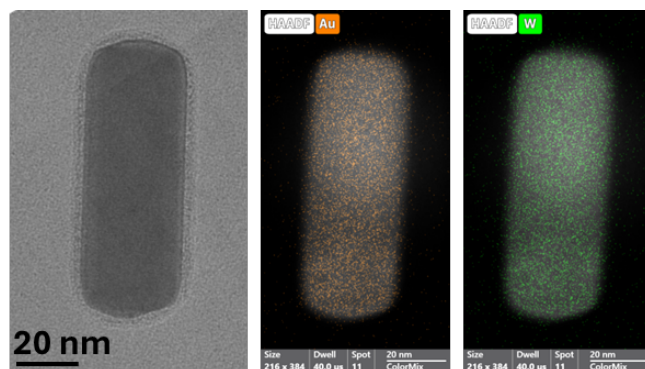
Figure 3. A TEM image (left) and elemental mapping of gold (middle) and tungsten (right) of the GNR-CTAB- POM1 structure, confirming the homogenous distribution of POM1 around the nanorod.
