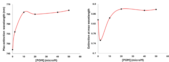
Figure 4. Monitoring changes in the maximum extinction wavelength (left) and extinction absorbance (right) of LSPR peak when POM1 (0, 2, 10, 20, 40, and 50 \mu\text{M} ) is added to GNRs (final concentration of GNRs in all samples is 0.1 nM), measured 1 hour after POM1 addition. The maximum extinction wavelength increases and then plateaus as the system becomes saturated with POM1 . The absorbance at the maximum extinction wavelength is observed to drop upon first addition of POM1 due to the formation of side-aggregates, rise as POM1 began to more fully coat the GNRs, and then reach a plateau point with excess POM1 .
