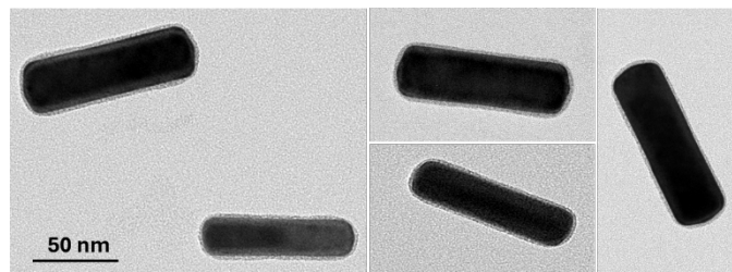
Figure 2. Transmission electron microscopy images of the GNR-CTAB- POM1 structure, revealing complete encapsulation of the GNR by the CTAB- POM1 monolayer. Additional images provided in the SI, Figure S2.
