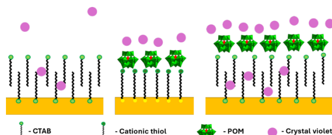
Scheme 3. Suggested location of crystal violet molecules relative to the GNR surface. Left: GNR-CTAB, in which the dye can sequester into the CTAB bilayer. Middle: GNR-MUTAB- POM1 in which the dye molecules are attracted to the negatively charged POM. Right: GNR-CTAB- POM1 which both attracts dye electrostatically and sequesters it.
