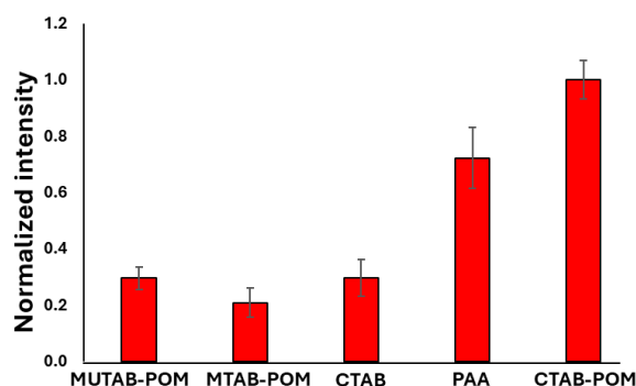
Figure 8. Raman signal intensity for crystal violet at 205 \text{cm}^{-1} obtained by differently functionalized GNR. The nanorod solutions used were all at a concentration of 0.1 nM.
