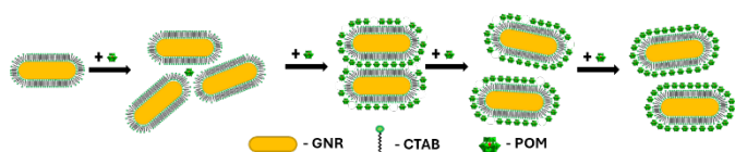
Scheme 2: Formation of the GNR-CTAB- POM1 structure. At low POM1 concentration the POM1 leads to unstable aggregation of GNRs. Higher POM1 concentration leads to stable aggregates, then no GNR aggregation and finally full POM1 coverage of the GNRs.
