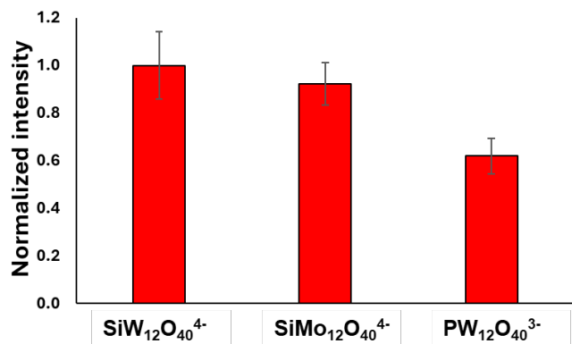
Figure 9. Raman signal of crystal violet at 205 cm -1 obtained by structures containing diff POM types. The nanorod solution used were all at a concentration of 0.1 nM.
