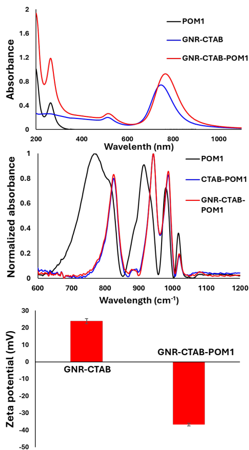
Figure 1. Top: UV-vis results for POM1 (0.1 mM), GNR-CTAB, and GNR-CTAB- POM1 (0.1 mM of POM1 ). After POM1 is added to the GNR-CTAB, a peak appears at 263 nm due to the presence of the POM, and the longitudinal and transverse plasmonic peaks red-shift and increase. Middle: FTIR results. The FTIR peaks red-shift when CTAB- POM1 complexes are formed. Peaks in the GNR-CTAB- POM1 structure are nearly identical to CTAB- POM1 , supporting the formation of GNR coated by CTAB and POM1 . Bottom: Zeta potential measurements. The surface charge of GNR is observed to change from positive to negative upon POM1 addition.
