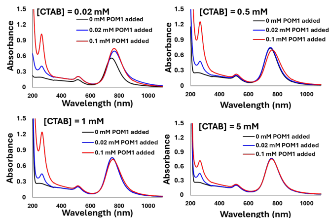
Figure 5. The addition of 0, 0.02 and 0.1 mM of POM1 to GNR-CTAB solutions containing total [CTAB] of 0.02, 0.5, 1 and 5 mM. As [CTAB] increases, the effect of POM1 addition on the SPR decreases.
