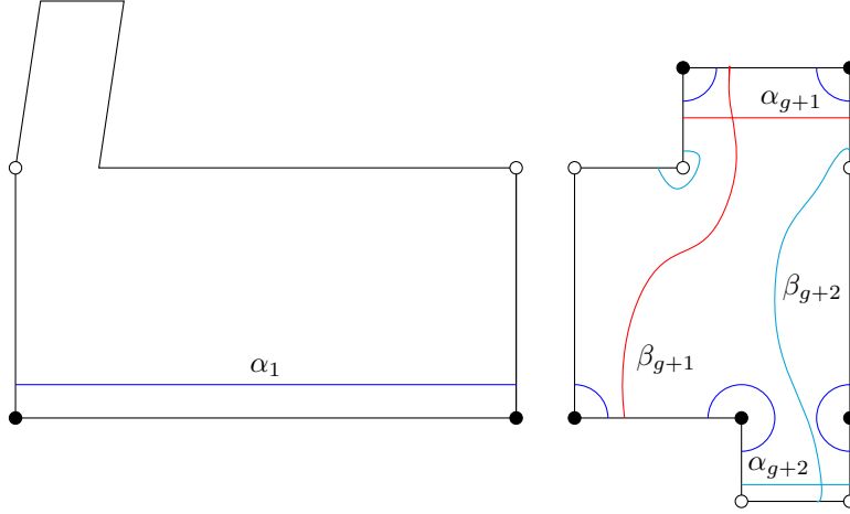
FIGURE 6. Modifying the symplectic basis, second case. Gluing as in Figure 4. Note the change in the rotation number of \beta_{g+2} .
