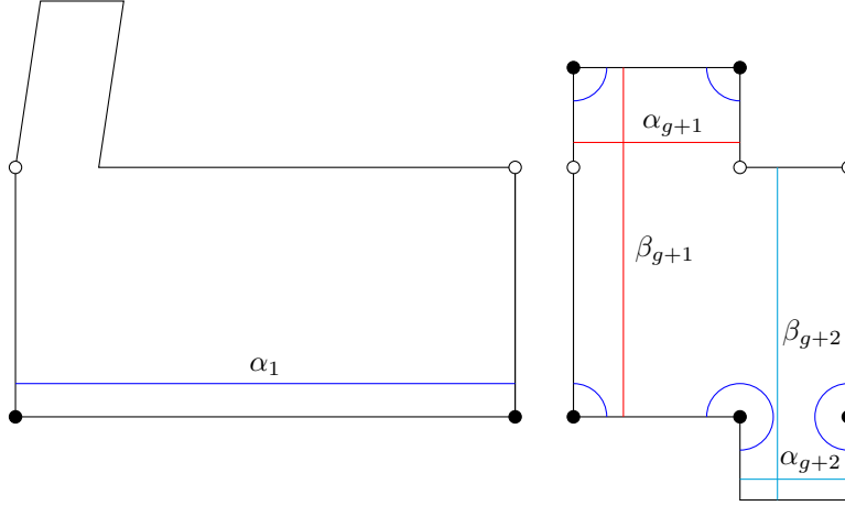
FIGURE 5. Modifying the symplectic basis. Gluing as in Figure 3
