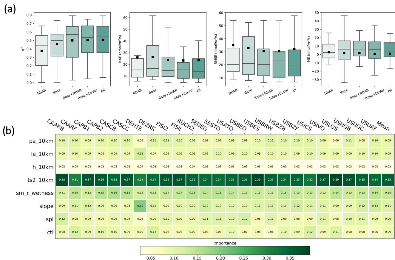
Figure 3. Grid-level modeling. Panel (a) presents the distribution of the R^2 , MAE, RMSE, and ME for all sites (size = 25) in a LOOCV scheme based on gridded data using five model settings: RF modeled using only MODIS NBAR bands, baseline features (MERRA-2 air pressure, latent heat flux, sensible heat flux, soil temperature, SMAP root zone soil wetness, topographic slope, spi, and cit), baseline features plus MODIS NBAR bands, baseline features plus correlated variables within the MERRA-2 and SMAP dataset, and all gridded input variables together. The model settings are ranked by the mean R^2 , from lowest (left) to highest (right). Panel (b) shows the mean variable importance of baseline models (last column) in the LOOCV scheme and at each site (columns labeled with validation site ID). The values in each column are the means of the accumulation of the impurity decrease when a variable was taken out in the trees of an RF model, representing the importance of such variable to the model. The variable names and descriptions refer to Table 1.
