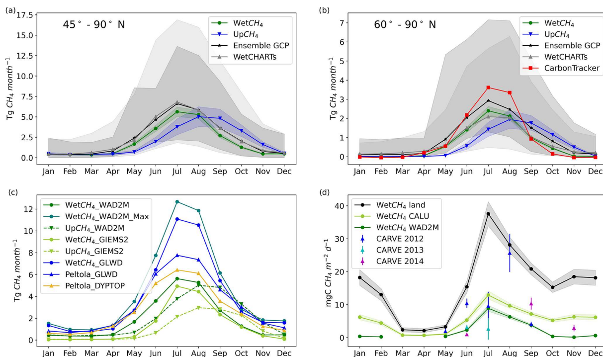
Figure 7. Multiyear average seasonal cycles of wetland CH 4 emissions. Panel (a) presents a comparison of ML upscaled mean seasonal cycles in reference wetland areas (WAD2Mv2) with the cycles from process-based models in the northern mid-high latitudes (45–90° N). Panel (b) shows the same comparison for northern high latitudes (60–90° N) and the addition of atmospheric CarbonTracker-CH 4 -attributed microbial emissions (2016–2022). Panel (c) presents a comparison of three ML upscaled mean seasonal cycles of CH 4 emissions with different wetland area maps (WAD2Mv2, WAD2Mv2 maximum extent, GIEMS2, and GLWDv1). Panel (d) shows a comparison of WetCH 4 mean seasonal cycles over land (black line), WetCH 4 weighted by wetland from the CALU map (light-green line), or WetCH 4 weighted by fractions from WAD2Mv2 (dark-green line), with estimates of CH 4 fluxes in growing seasons from CARVE retrievals in the North Slope area of Alaska (Zona et al., 2016).
