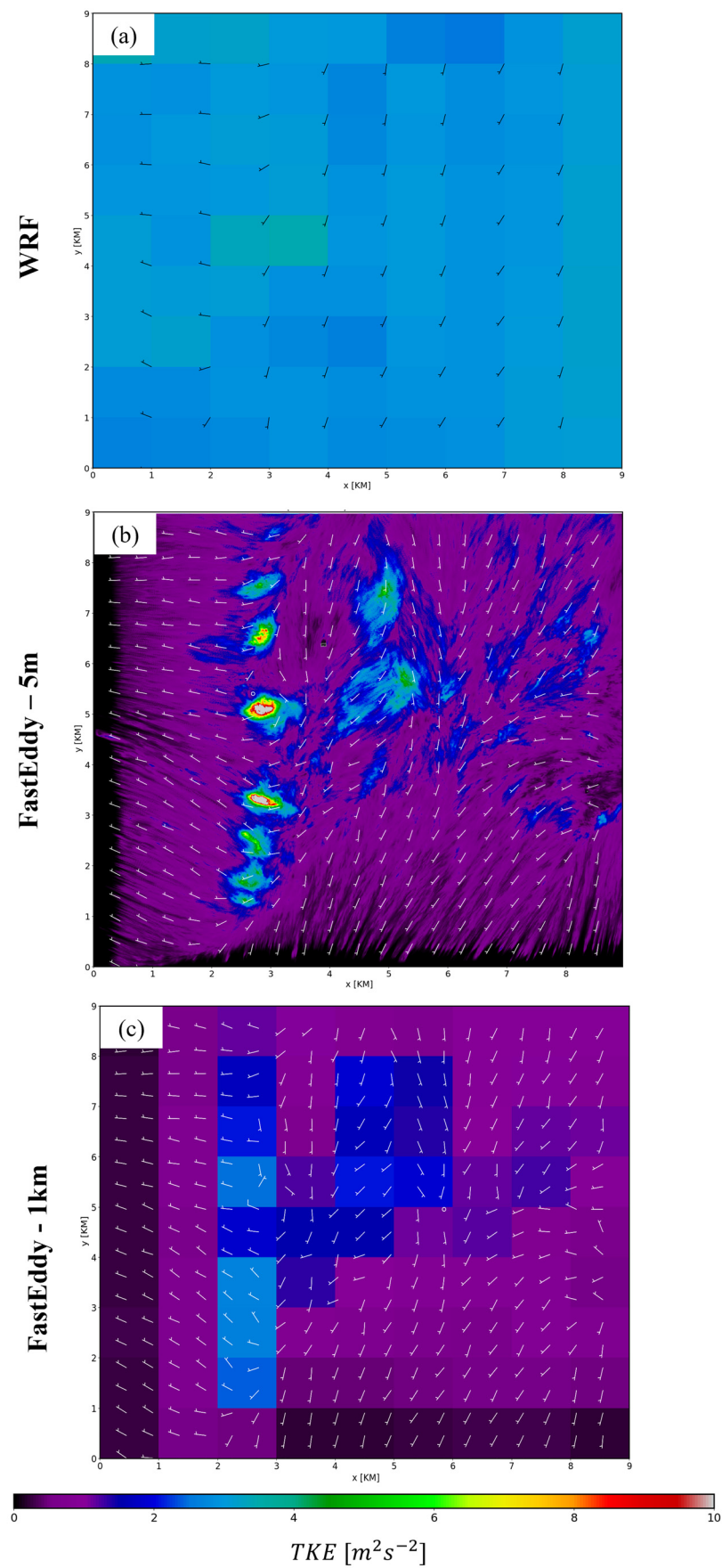
Figure 13. TKE ( m^2 s^{-2} , shaded) at 30 m AGL at 17:30 UTC: (a) WRF; (b) FE; and (c) FE upscaled to 1 km. Vector winds plotted as in earlier figures.
