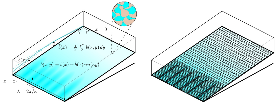
Figure 1. Left, the geometry used in this paper, showing the ice divide at x = 0 , the terminus as x_t , and an example gap height distribution b(x, y) (color), with width-average \bar{b}(x) = \frac{1}{Y} \int_0^Y b(x, y) dy and variation of size \hat{b}(x) at a wavelength \lambda . The spatial structure of pressure head and flux is similarly decomposed into an average plus a periodic perturbation. Away from channels, the effective gap height b represents a local average over flow through connected cavities (inset). Right, a schematic showing mesh refinement in the numerical simulations, with finer meshes in areas of higher spatial variability. Each step in refinement halves the grid size. Both the minimum and maximum levels of refinement can be set manually and we use up to 10 levels (compared to the 3 shown here). Only perturbations where \lambda is at least twice the minimum grid size can be resolved numerically.
