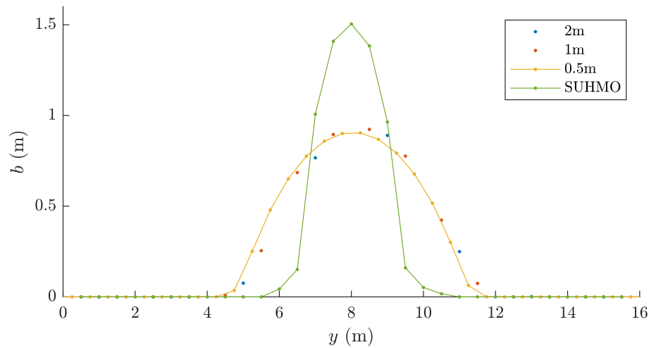
Figure A1. Gap height b at a transect 10 m inland of the margin, when a large moulin is located 16 m inland of the margin. We see convergence in channel width and height with increasing resolution. The same example in SUHMO produces a taller, narrower channel, as expected.
