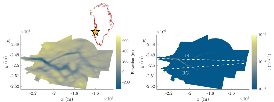
Figure 9. (a) Topography beneath Russell Glacier (RG) and Isunnguata Sermia (IS). The inset shows the location in southwest Greenland. (b) Subglacial water flux beneath RG and IS under winter conditions, as simulated in SHAKTI. A channel develops beneath IS following the lows in basal topography (Morlighem et al., 2017). Dashed lines indicate the profiles of topography and ice thickness used for the stability calculations.
