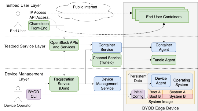
Figure 1: Interactions between the architectural roles and components of CHI@Edge.
