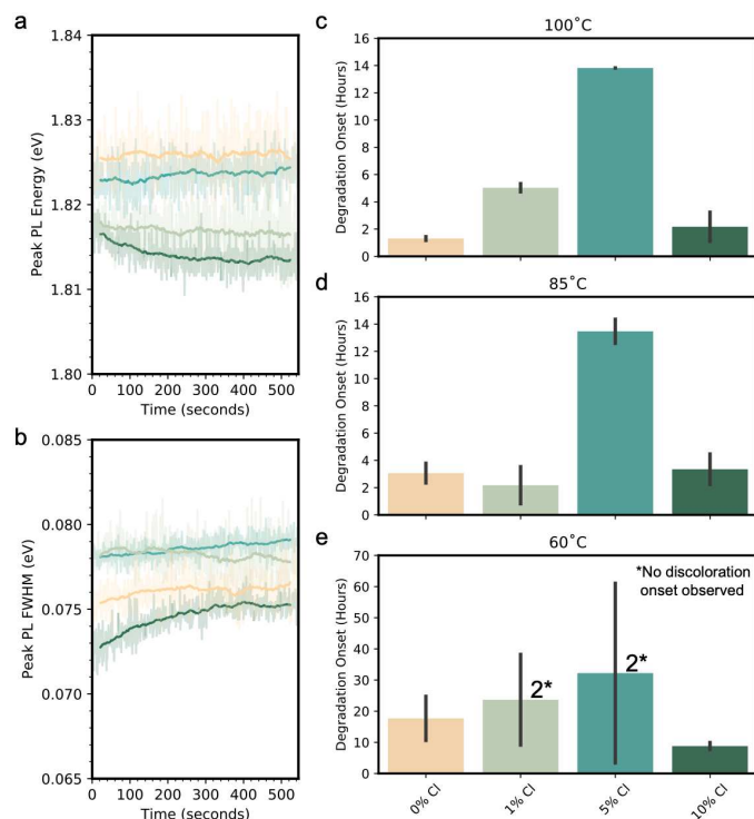
Fig. 5 (a) Peak PL emission energy and PL FWHM (b) of \text{CsPb}(\text{I}_{0.80}\text{Br}_{0.20-x}\text{Cl}_x)_3 films collected from a single point ( 6\mu\text{m} ) over 545s. Raw data is in lighter color (yellow is 0% Cl, light green is 1% Cl, teal is 5% Cl, and 10% Cl is dark green) with 100s rolling average in darker color. Bar plots of fitted onset of discoloration of \text{CsPb}(\text{I}_{0.80}\text{Br}_{0.20-x}\text{Cl}_x)_3 of films held at (c) 100°C, (d) 85°C, and (e) 60°C, black bar indicates respective standard deviation. For samples where no discoloration onset was observed, the onset of discoloration was conservatively estimated as the final test time. Bars encompassing such samples have the count of occurrences denoted by a number, accompanied by an asterisk, placed above them. A total of 2 samples per condition were observed for 100°C and 85°C temperatures, with 4 samples observed for 60°C.
