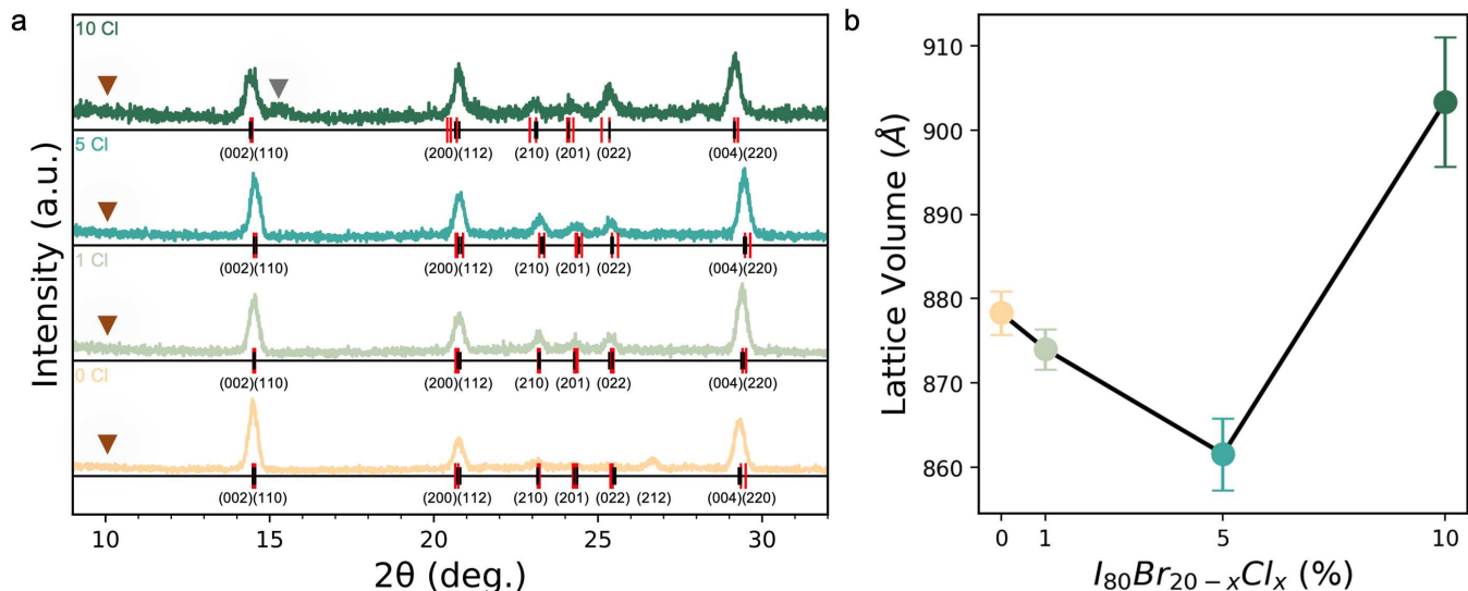
Fig. 1 a) Parallel beam thin film diffraction XRD of CsPb(I_{0.80}Br_{0.20-x}Cl_x)_3 films with Cl varied from 0% to 10%. The orthorhombic (Pnma) calculated peaks are marked as red vertical lines, with observed two theta peak location as black vertical lines. Emerging secondary phase in 10% Cl marked with gray arrow and the location of the non-perovskite \delta -phase peak were it to be present marked by the brown triangle. 8.04keV X-ray source. b) Lattice volume calculated from DICVOL14 based on orthorhombic indexing.
