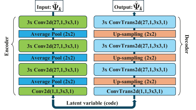
Fig. 2. Autoencoder design for centralized radiomap estimation.
