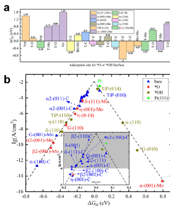
Figure 6. (a) Free-energy change of adsorbed H ( \Delta G_H ) on different sites of O* and HO* surfaces. \delta , \alpha , G, \eta , TiP refer to different Mo x C crystal phases and structures. (b) Exchange current densities as a function of hydrogen adsorbed free energy for MoC and Mo 2 C surfaces. The grey area indicates the corresponding surfaces which exhibit an exchange current density larger than 0.1 mA/cm 2 . \alpha 2 and \beta 2 represents \alpha -MoC and \beta -Mo 2 C, respectively. Reprinted with permission from Ref. [11].
