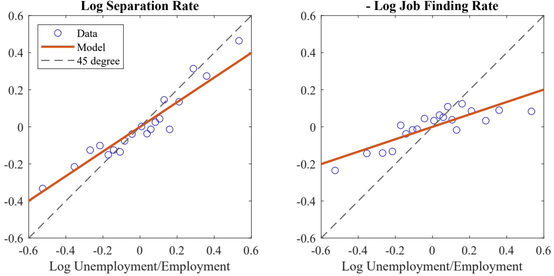
Notes: Decomposition of local unemployment rate differences in the model and data into differences of separation and job-finding rates. The left panel shows the (demeaned) log separation rate from the model (red line) and from the data (blue circles) against the (demeaned) log unemployment-employment ratio (horizontal axis). The right panel shows the negative (demeaned) log job-finding rate from the model (red line) and from the data (blue circles). The dashed gray line in each panel shows the 45 degree line. The data points are from from Figure 7.
