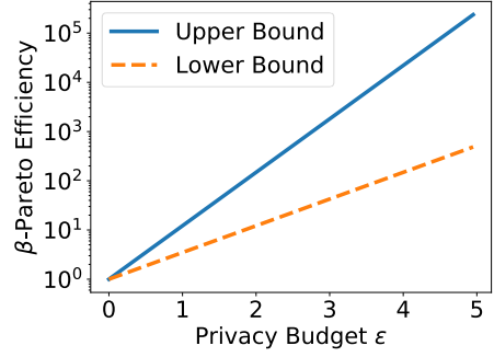
Figure 1: Tradeoff curves (upper and lower bounds) between \beta -PE and \epsilon -DP, where m = 5, n = 10 .
