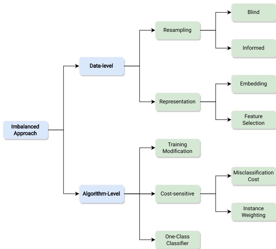
Fig. 2 Taxonomy of approaches for imbalanced data streams
