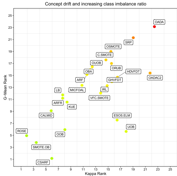
Fig. 26 Comparison of all 24 algorithms for concept drift with increasing class imbalance ratio. Color gradient represents the product of both metrics (Color figure online)
