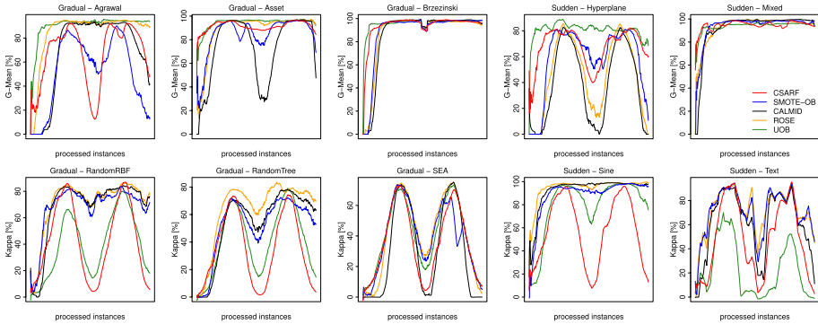
Fig. 9 G-Mean and Kappa on flipping and refliping class imbalance ratio with gradual and sudden drift
