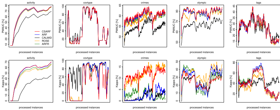
Fig. 41 PMAUC and Kappa on semi-synthetic multi-class imbalanced datasets
