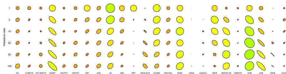
Fig. 5 Comparison of all 24 algorithms for different levels of static class imbalance ratio. The axes of the ellipse represent G-Mean and Kappa metrics. The bigger the axes the better rank of the algorithm on the metrics. The more rounded the ellipse the more agreement between the metrics. The color gradient represents the product of both metrics' ranks (Color figure online)
