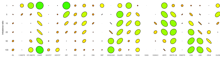
Fig. 20 Comparison of all 24 algorithms for merging minority clusters on static class imbalance ratio. Axes of the ellipse represent G-Mean and Kappa metrics. Color gradient represents the product of both metrics (Color figure online)
