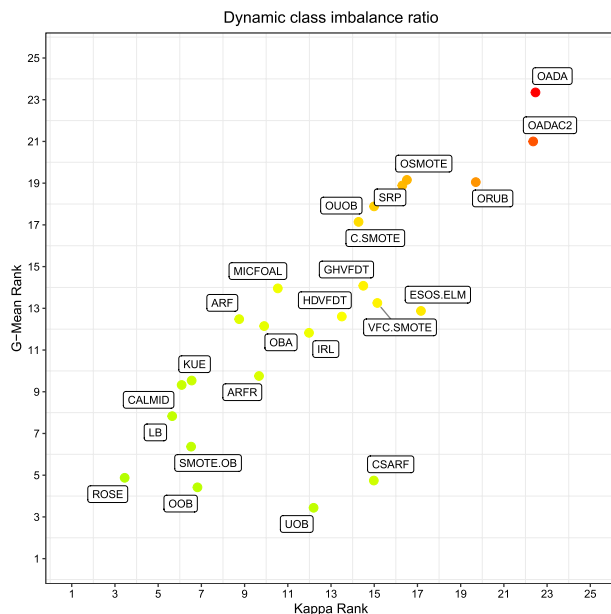
Fig. 10 Comparison of all 24 algorithms for dynamic class imbalance ratio. Color gradient represents the product of both metrics (Color figure online)
