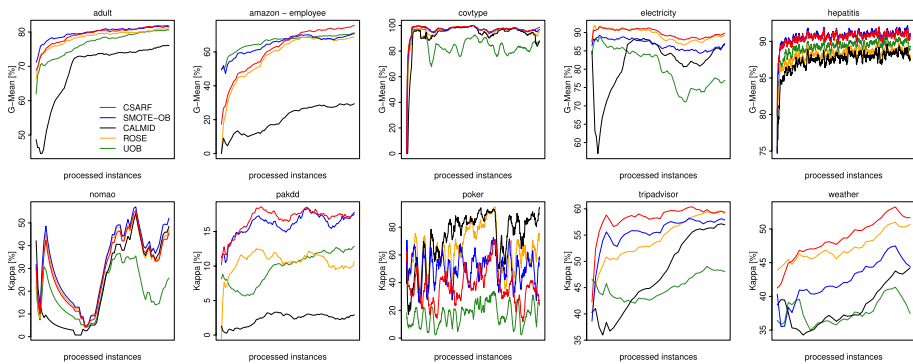
Fig. 27 G-Mean and Kappa on binary class imbalanced datasets
