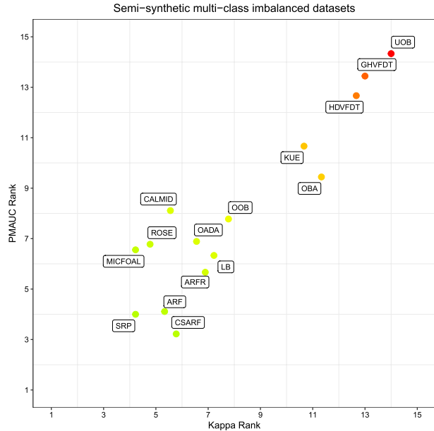
Fig. 42 Comparison of all 15 algorithms for semi-synthetic multi-class imbalanced datasets. Color gradient represents the product of both metrics (Color figure online)
