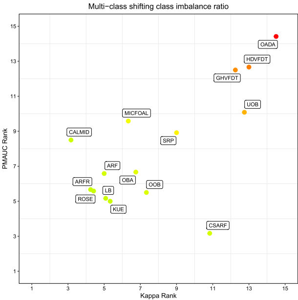
Fig. 32 Comparison of all 15 algorithms for multi-class shifting class imbalance ratio. Color gradient represents the product of both metrics (Color figure online)
