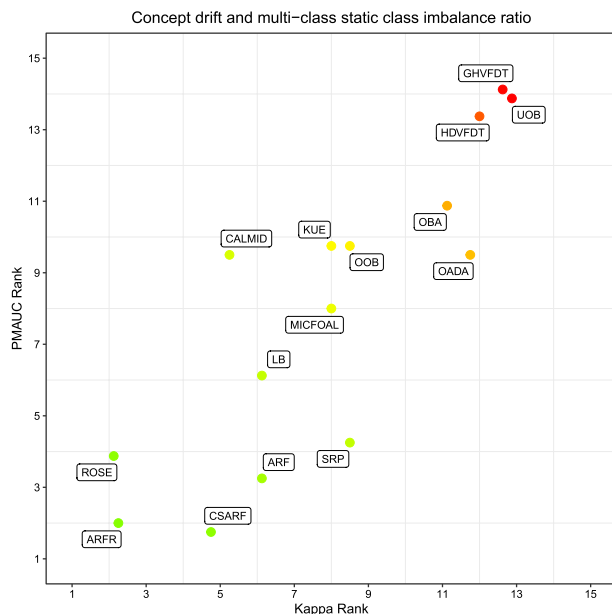
Fig. 34 Comparison of all 15 algorithms on concept drift and multi-class static class imbalance ratio. Color gradient represents the product of both metrics
