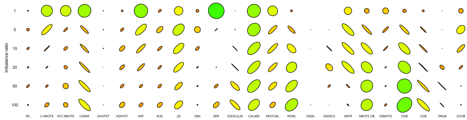
Fig. 16 Comparison of all 24 algorithms for borderline instances on static class imbalance ratio. Axes of the ellipse represent G-Mean and Kappa metrics. Color gradient represents the product of both metrics (Color figure online)
