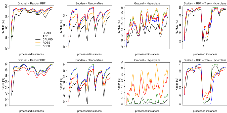
Fig. 33 PMAUC and Kappa on concept drift and multi-class static imbalance ratio
