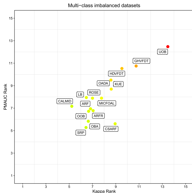
Fig. 40 Comparison of all 15 algorithms for multi-class imbalanced datasets. Color gradient represents the product of both metrics (Color figure online)
