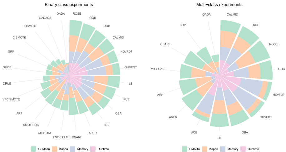
Fig. 45 Overall comparison of stacked algorithms' ranks for G-Mean/PMAUC, Kappa, runtime, and memory on binary and multi-class imbalanced benchmarks. Algorithms are sorted clockwise by the stacked ranks best to worst. Equal weight for the four metrics
