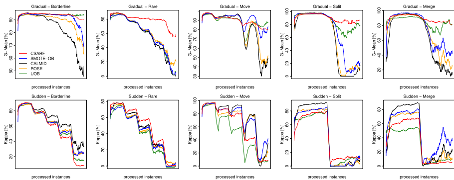
Fig. 21 G-Mean and Kappa on increasing borderline, rare, moving, splitting, and merging minority clusters and increasing imbalance ratio
