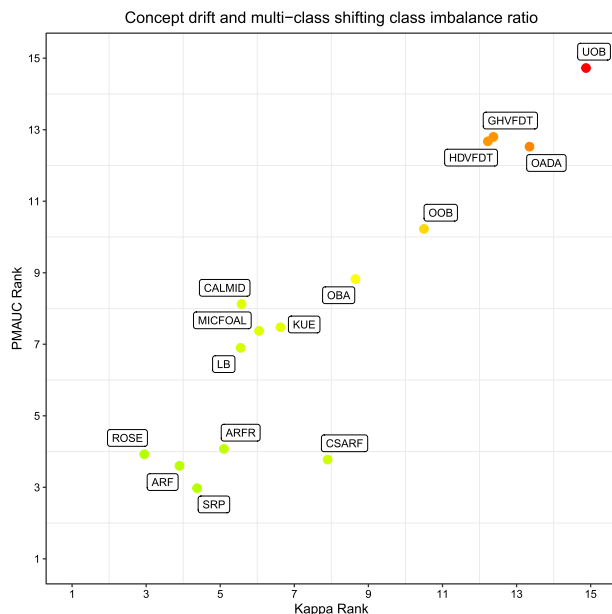
Fig. 36 Comparison of all 15 algorithms on concept drift and multi-class shifting class imbalance ratio. Color gradient represents the product of both metrics (Color figure online)
