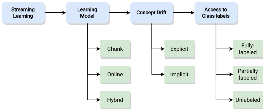
Fig. 1 Streaming learning taxonomy
