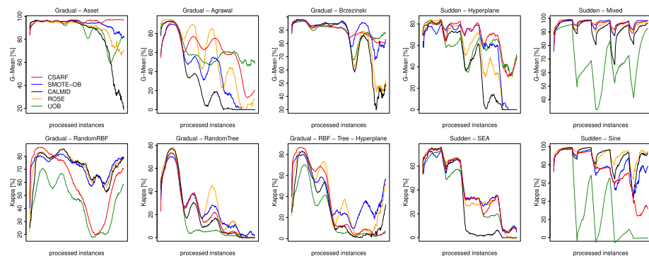
Fig. 25 G-Mean and Kappa on concept drift with increasing imbalance ratio
