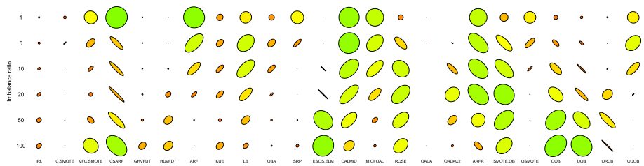
Fig. 18 Comparison of all 24 algorithms for moving minority clusters on static class imbalance ratio. Axes of the ellipse represent G-Mean and Kappa metrics. Color gradient represents the product of both metrics (Color figure online)
