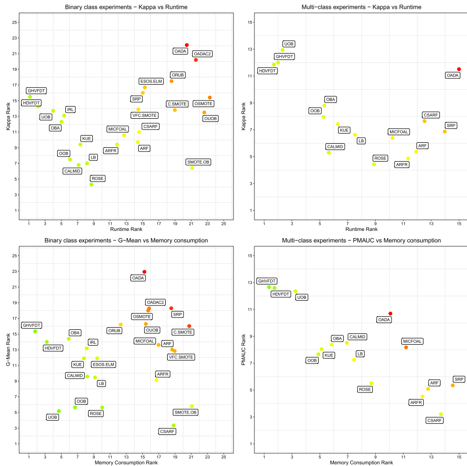
Fig. 44 Overall comparison of algorithms' ranks for G-Mean/PMAUC/Kappa versus Runtime/Memory Consumption on binary and multi-class imbalanced benchmarks. Color gradient represents the product of each pair of metrics (Color figure online)
