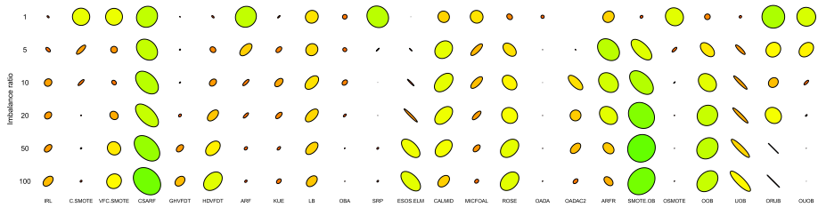
Fig. 17 Comparison of all 24 algorithms for rare instances on static class imbalance ratio. Axes of the ellipse represent G-Mean and Kappa metrics. Color gradient represents the product of both metrics (Color figure online)
