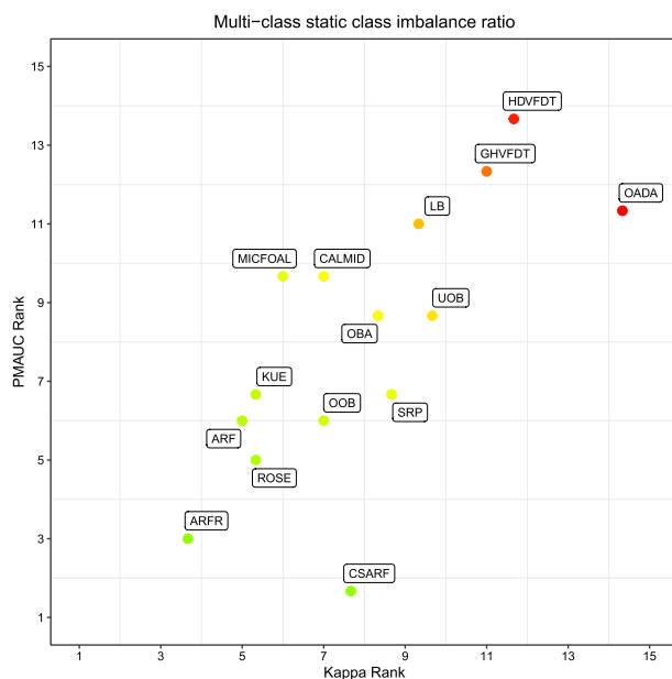
Fig. 30 Comparison of all 15 algorithms for multi-class static class imbalance ratio. Color gradient represents the product of both metrics (Color figure online)
