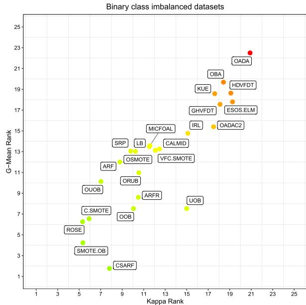
Fig. 28 Comparison of all 24 algorithms for binary class imbalanced datasets. Color gradient represents the product of both metrics (Color figure online)
