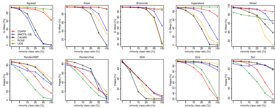
Fig. 4 Robustness to different levels of static class imbalance ratio (G-Mean and Kappa)
