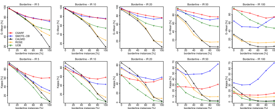
Fig. 11 Robustness to borderline instances for static imbalance ratio (G-Mean and Kappa)
