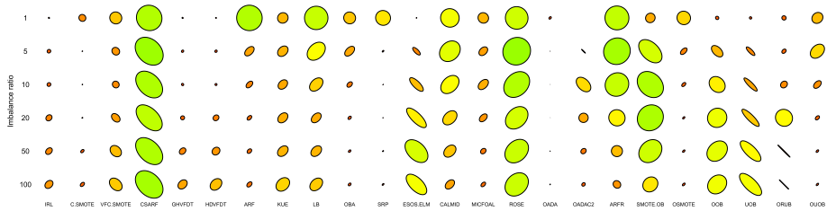
Fig. 24 Comparison of all 24 algorithms for concept drift with static class imbalance ratio. Axes of the ellipse represent G-Mean and Kappa metrics. Color gradient represents the product of both metrics (Color figure online)
