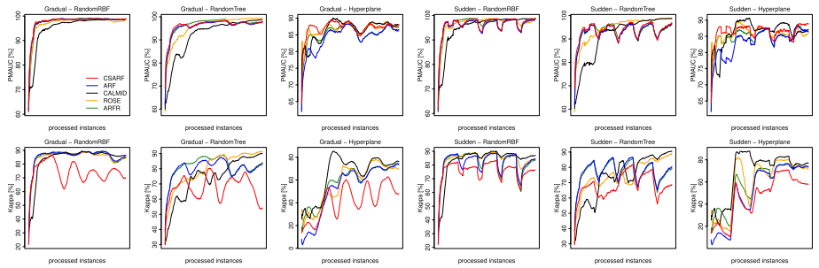
Fig. 31 PMAUC and Kappa on multi-class shifting imbalance ratio
