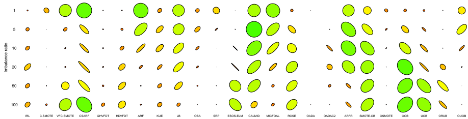
Fig. 19 Comparison of all 24 algorithms for splitting minority clusters on static class imbalance ratio. Axes of the ellipse represent G-Mean and Kappa metrics. Color gradient represents the product of both metrics (Color figure online)
