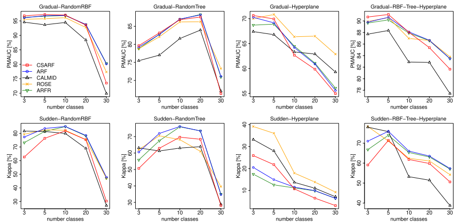
Fig. 37 Impact of the number of classes on PMAUC and Kappa under concept drift and multi-class shifting imbalance ratio
