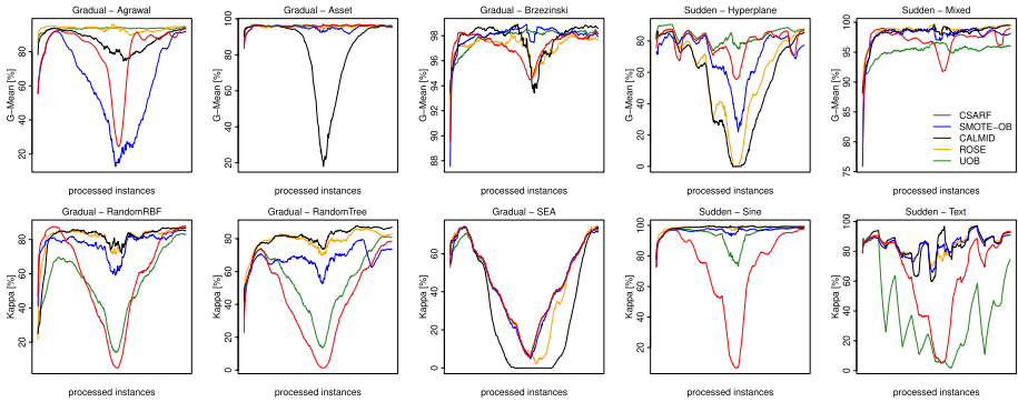
Fig. 7 G-Mean and Kappa on increasing decreasing class imbalance ratio with gradual and sudden drift
