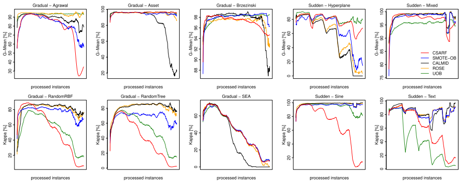
Fig. 6 G-Mean and Kappa on increasing class imbalance ratio with gradual and sudden drift
