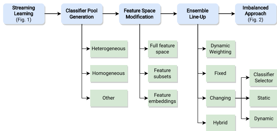
Fig. 3 Taxonomy of ensemble definition for imbalanced data streams
