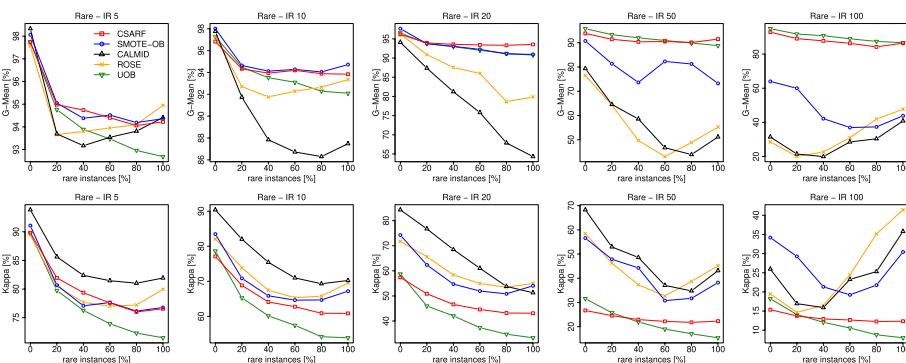
Fig. 12 Robustness to rare instances for static imbalance ratio (G-Mean and Kappa)
