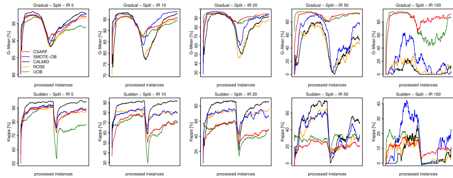
Fig. 14 G-Mean and Kappa on splitting minority clusters for static imbalance ratio
