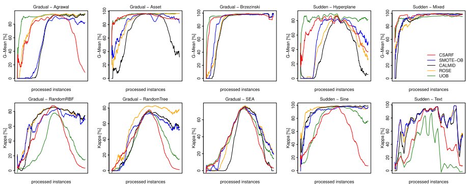
Fig. 8 G-Mean and Kappa on flipping class imbalance ratio with gradual and sudden drift
