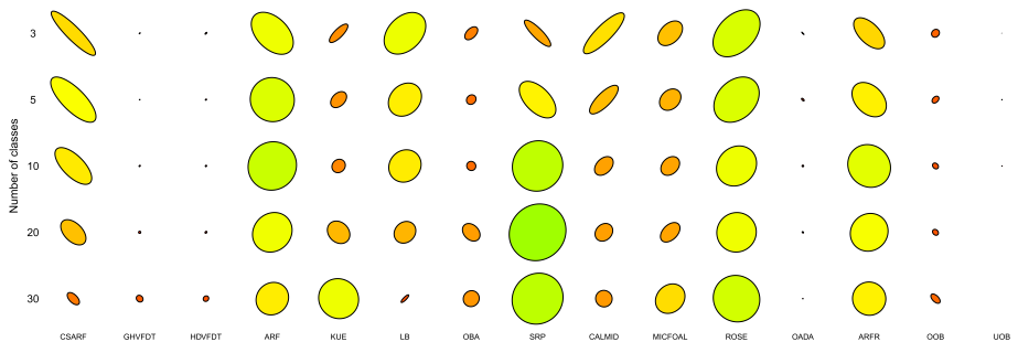
Fig. 38 Comparison of all 15 algorithms on the number of classes under concept drift and multi-class shifting imbalance ratio. Axes of the ellipse represent PMAUC and Kappa metrics. Color gradient represents the product of both metrics (Color figure online)
