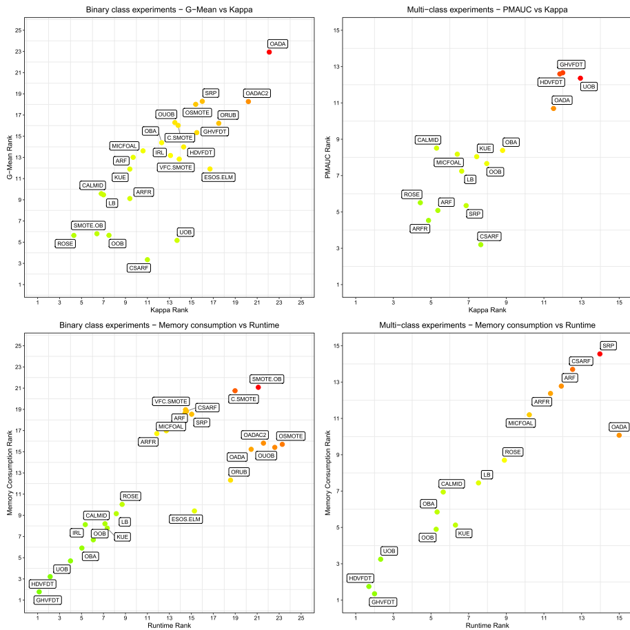
Fig. 43 Overall comparison of algorithms' ranks for G-Mean/PMAUC versus Kappa and Memory Consumption versus Runtime on binary and multi-class imbalanced benchmarks. Color gradient represents the product of each pair of metrics (Color figure online)
