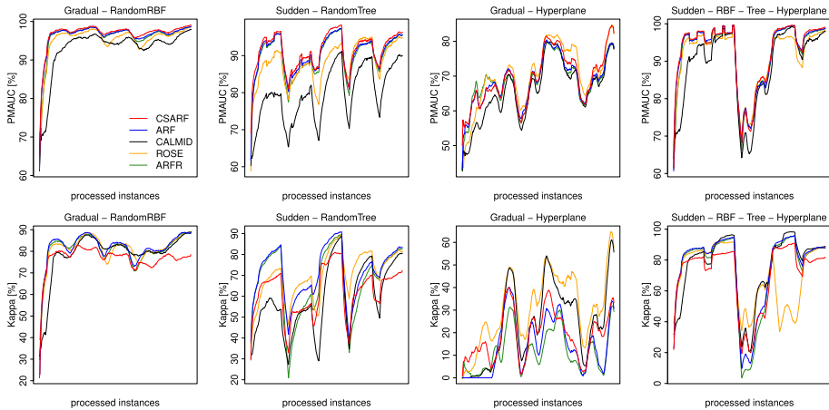
Fig. 35 PMAUC and Kappa on concept drift and multi-class shifting imbalance ratio
