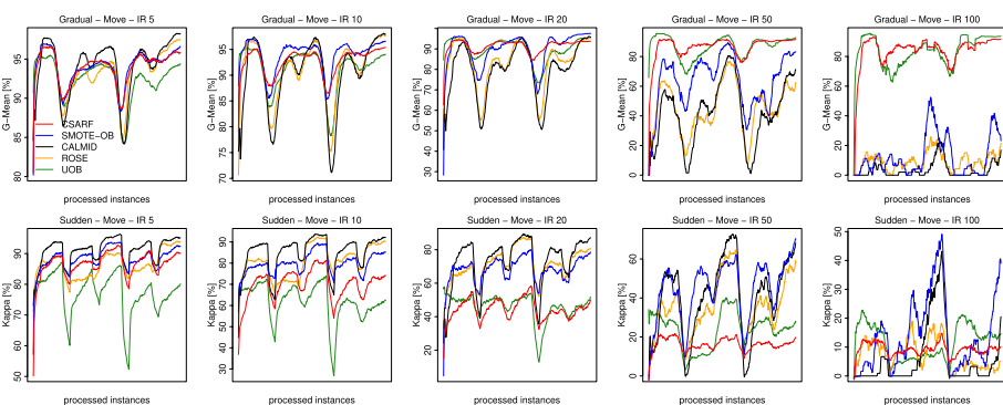
Fig. 13 G-Mean and Kappa on moving minority clusters for static imbalance ratio
