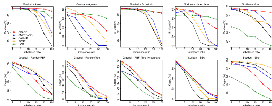
Fig. 23 Robustness to concept drift with static class imbalance ratio (G-Mean and Kappa)
