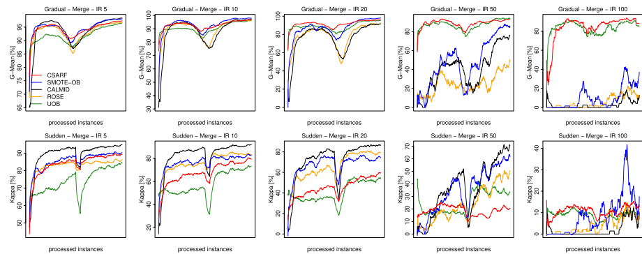
Fig. 15 G-Mean and Kappa on merging minority clusters for static imbalance ratio
