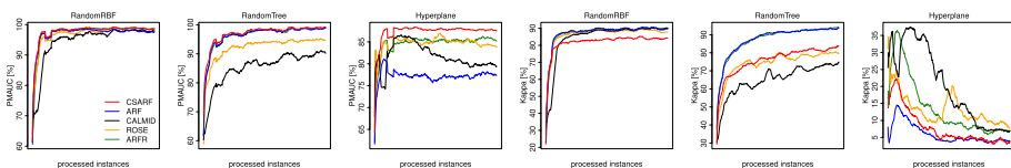
Fig. 29 PMAUC and Kappa on multi-class static imbalance ratio
