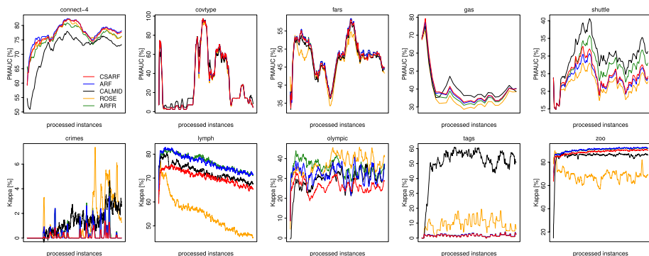
Fig. 39 PMAUC and Kappa on multi-class imbalanced datasets
