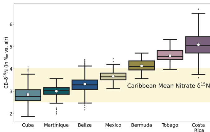
Extended Data Fig. 2 | Coral-bound \delta^{15}\text{N} distribution across the Wider Caribbean. Boxplots based on 2507 newly measured \text{CB-}\delta^{15}\text{N} values (in ‰ vs. air) grouped according to the coral core location and compared to the mean Caribbean nitrate \delta^{15}\text{N} ( 3.28 \pm 0.76\text{‰} ) as indicated by the horizontal shaded area. \text{CB-}\delta^{15}\text{N} values for Bermuda are based on Wang et al. (2015). Values above mean Caribbean nitrate \delta^{15}\text{N} indicate regions that are suspected to be influenced by local conditions. The white dot represents the average value whereas the
