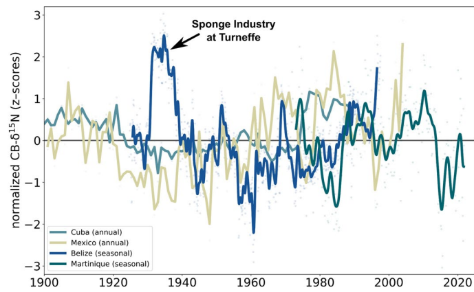
Extended Data Fig. 3 | Normalized (z-scores) CB- \delta^{15}\text{N} timeseries. The compilation is based on the measured coral cores that were used for the stacked record. Raw CB- \delta^{15}\text{N} values were standard score normalized (z-score) according to the normalized CB- \delta^{15}\text{N} = [(\text{CB-}\delta^{15}\text{N} - \text{average CB-}\delta^{15}\text{N}) / (\text{standard deviation of CB-}\delta^{15}\text{N})] . A Gaussian smoothing was applied to each CB- \delta^{15}\text{N} timeseries to highlight the low-frequency shared natural variability between each location.
