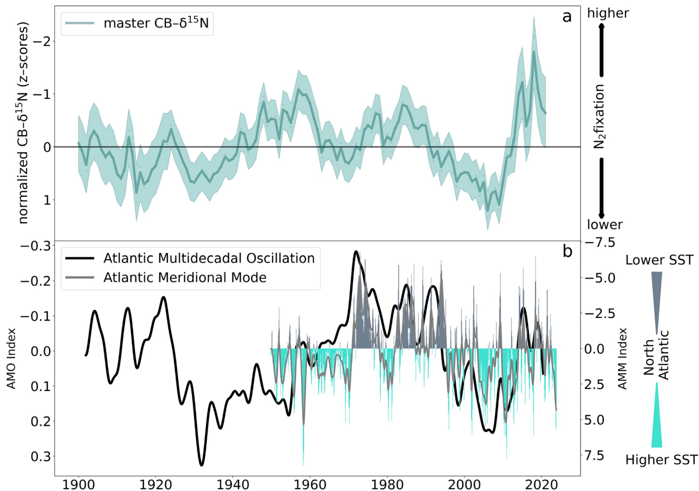
Extended Data Fig. 7 | Coral-bound \delta^{15}\text{N} master record versus AMO and AMM index. a , The stacked normalized \text{CB-}\delta^{15}\text{N} record in relation to the b , Atlantic Meridional Mode index based on Chiang and Vimont, 2004 2 . The Atlantic Multidecadal Oscillation is superimposed to show interrelations. Positive AMM
