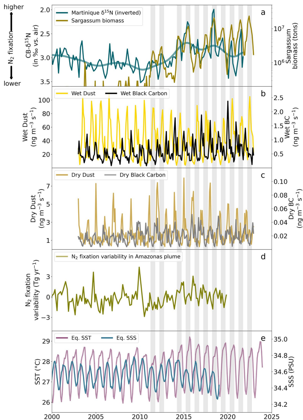
Extended Data Fig. 9 | Martinique \text{CB-}\delta^{15}\text{N} record and alternative environmental parameters used to explain Sargassum blooms. a , \text{CB-}\delta^{15}\text{N} values (in ‰ vs. air) of the coral core taken from Martinique in relation to the logarithmic Sargassum spp. biomass of the equatorial Atlantic and Caribbean ( 0\text{--}20^{\circ}\text{N} , 40\text{--}90^{\circ}\text{W} ). b , Area weighed ( 10\text{--}20^{\circ}\text{N} , 20\text{--}60^{\circ}\text{W} ) dry dust and dry black carbon deposition ( \text{ng m}^{-3} \text{s}^{-1} ), calculated with the EMAC model
