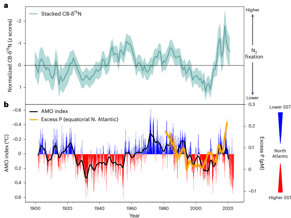
Fig. 2 | CB- \delta^{15}\text{N} master record and comparison to the AMO. a , The normalized master CB- \delta^{15}\text{N} record (z scores) with the propagated error ( \pm 1\text{s.d.} , shaded region) is based on four coral cores (Belize, Cuba, Martinique and Mexico from 1900 to 2021) from the wider Caribbean region and is closely related to Caribbean nitrate \delta^{15}\text{N} . Higher normalized CB- \delta^{15}\text{N} values correspond to lower rates of \text{N}_2 fixation, whereas lower normalized CB- \delta^{15}\text{N} values are indicative of higher \text{N}_2 fixation rates. b , Compared with a is the AMO index derived from Trenberth and Shea 52 (black line) and the locally estimated scatterplot smoothing (LOESS) of
