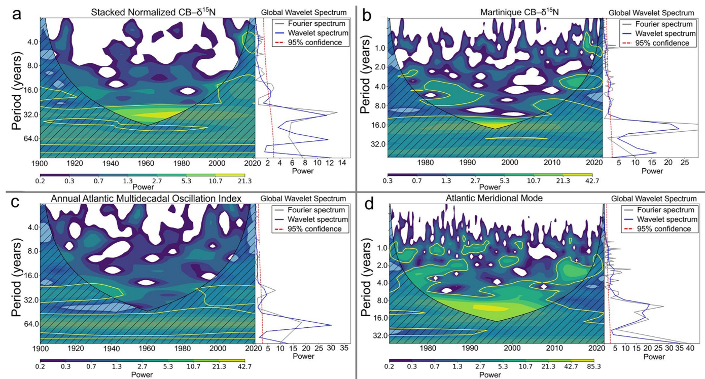
Extended Data Fig. 4 | Continuous Wavelet Transformation plot of the master CB-\delta^{15}N record and the AMO as well Martinique CB-\delta^{15}N record and the AMM. a, Continuous Wavelet Transformation plot and Cross Wavelet Analysis of the normalized master CB-\delta^{15}N and b, the CB-\delta^{15}N record from Martinique versus c,
