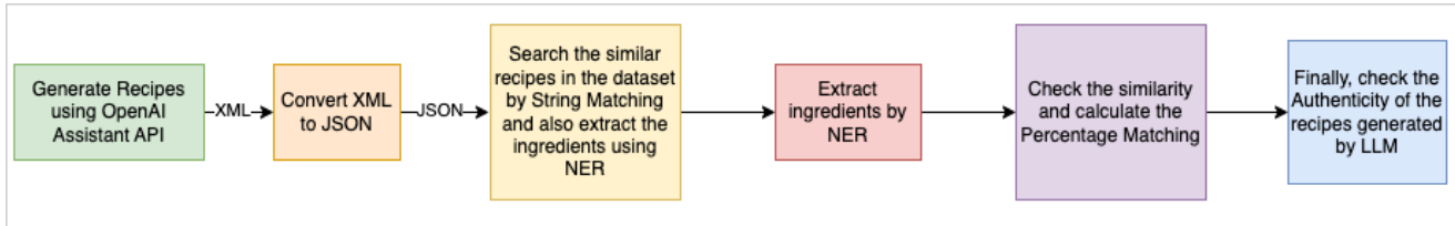
Fig. 1. Processing pipeline for evaluating recipes.
