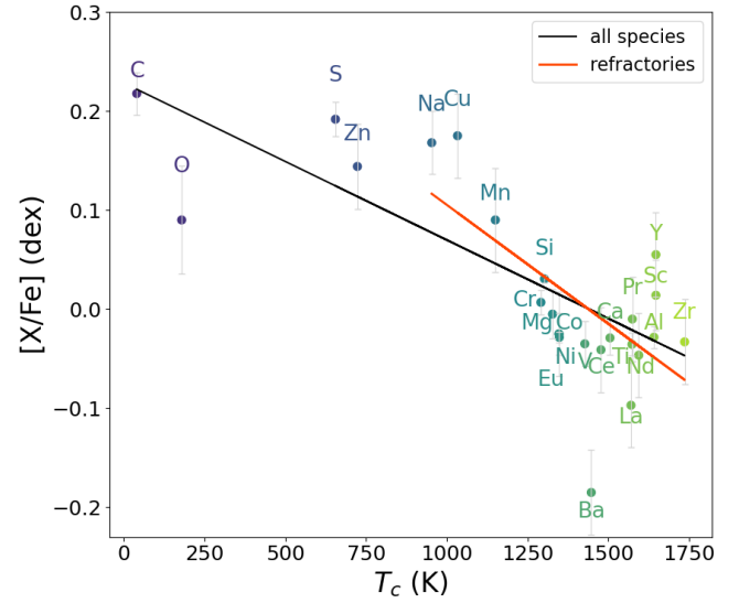
Fig. 2. Differential abundances from Krios–Kronos vs. T_{\text{C}} . The weighted linear fits to all elements and to refractories are represented as a black and a red line, respectively.
