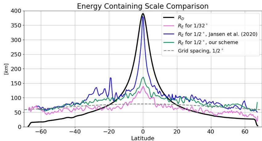
Figure 12. Zonally and 500-day averaged deformation scale (for 1/32° case) and energy-containing scale for the 1/32° case, 1/2° case with the Jansen et al. (2020) scheme, and our 1/2° backscatter case. Grid spacing for the 1/2° simulations is shown in dashed gray.
